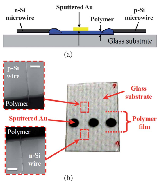
Fig. 2 (a) Schematic diagram of the measurement system. This system was used as a representation for the photoelectrochemical device depicted in Fig. 1. The PEDOT:PSS:Nafion film (~200 nm thick) was spin-coated onto a glass substrate. H-terminated and CH 3 -terminated p-type and n-type Si microwires were aligned at the polymer/glass border, with 2–5 μm of the microwire embedded into the polymer. Au contacts (32 nm thick) were sputtered onto the polymer to provide ohmic contacts to the polymer membrane; (b) photograph of the test structure, along with SEM micrographs of the microwires aligned at each side. SEM images were taken on a gold-coated slide to minimize charging issues. The scale bars in the images are 20 μm.
