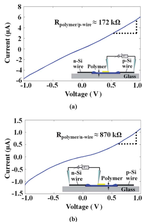
Fig. 3 I – V data for a 100 μm long freshly etched (a) H-terminated p-type Si microwire and (b) H-terminated n-type Si microwire, both with diameters of ~1.5 μm aligned at the PEDOT:PSS:Nafion/glass border (figure insets). The total series resistance of the system in each case (displayed in the figures) was used to extract the junction resistance, R_{C-p} or R_{C-n} , by incorporating the known values of R_{wire} and R_{polymer} .
