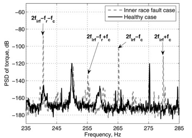
Figure 4 Spectrum of mechanical load torque – comparison between healthy and inner race fault cases
