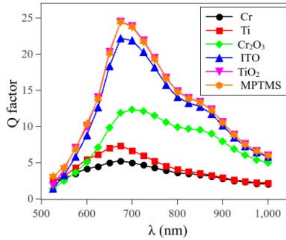
Figure 13: Q-factor of nanospheres of a mixture of gold and adhesion layer material.
