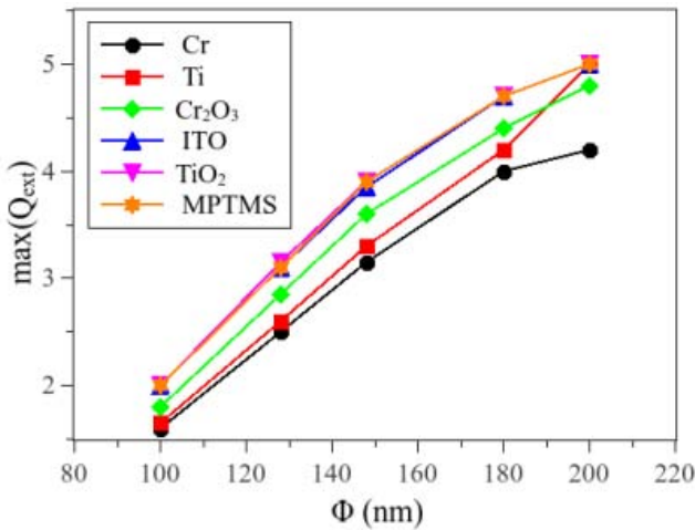
Figure 5: Maximum extinction efficiency as a function of the diameter.
