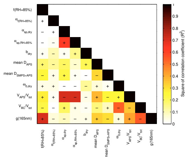
Fig. 3. Correlation plot of all intensive aerosol parameters measured in-situ at the Cabauw tower. f(\text{RH}=85\%, 550\text{ nm}) : scattering enhancement factor; \alpha_{f(\text{RH})} : Ångström exponent of f(\text{RH}=85\%, 550\text{ nm}) ; \alpha_{\text{sp,dry}} : Ångström exponent of scattering coefficient at low RH; \alpha_{\text{sp,RH}=85\%} : Ångström exponent of scattering coefficient at \text{RH}=85\% ; b_{\text{dry}} : backscatter fraction (at \lambda=550\text{ nm} ) at low RH; D_{\text{APS}} : mean (dry) diameter of APS size distribution measurement; D_{\text{SMPS}} : mean (dry) diameter of SMPS size distribution measurement; \omega_{0,\text{dry}} : single scattering albedo at low RH (at \lambda=550\text{ nm} ); V_{\text{APS}}/V_{\text{tot}} : coarse mode fraction measured by APS and SMPS; V_{\text{BC}}/V_{\text{tot}} : black carbon volume fraction measured by MAAP, SMPS, and APS; g(\text{RH}=90\%, 165\text{ nm}) : hygroscopic growth factor measured at the dry diameter d_0=165\text{ nm} and at \text{RH}=90\% by the H-TDMA. Plus and minus signs indicate the slope of the regression line.
