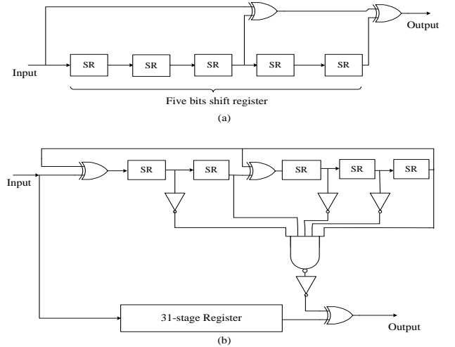
Fig. 3. Nonsystematic encoder [35] (a) and Meggit decoder (b) [35] for m = 5 Hamming code.
