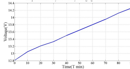
Fig. 2: Charging of Lead Crystal Batter via Solar Panel
