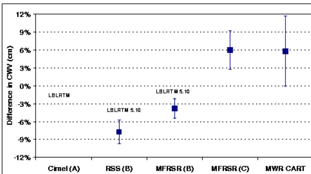
Figure 2. Same as Figure 1 but LBLRTM 5.10 has been used for methods A and B. The Cimel data are not available yet.
