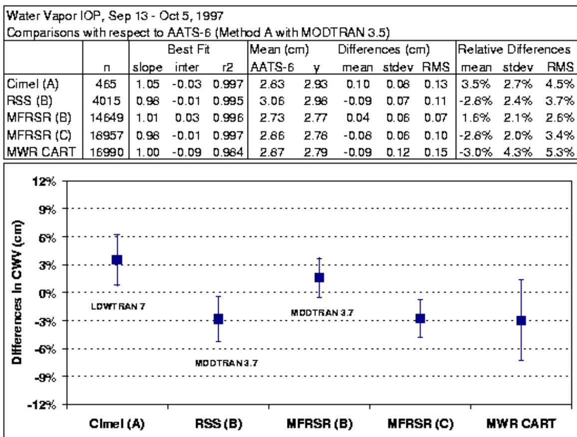
Figure 1. Comparison of CWV from different instruments and methods to AATS-6. This is the initial comparison where different radiative transfer models (as indicated) have been used.
