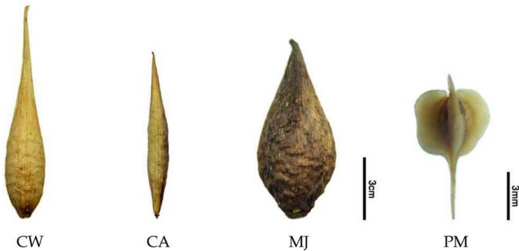
Fig. 7. Fruit shape of Cynanchum wilfordii , C. auriculatum , Metaplexis japonica and Polygonum multiflorum . CW; Cynanchum wilfordii , CA; C. auriculatum , MJ; Metaplexis japonica , PM; Polygonum multiflorum .
