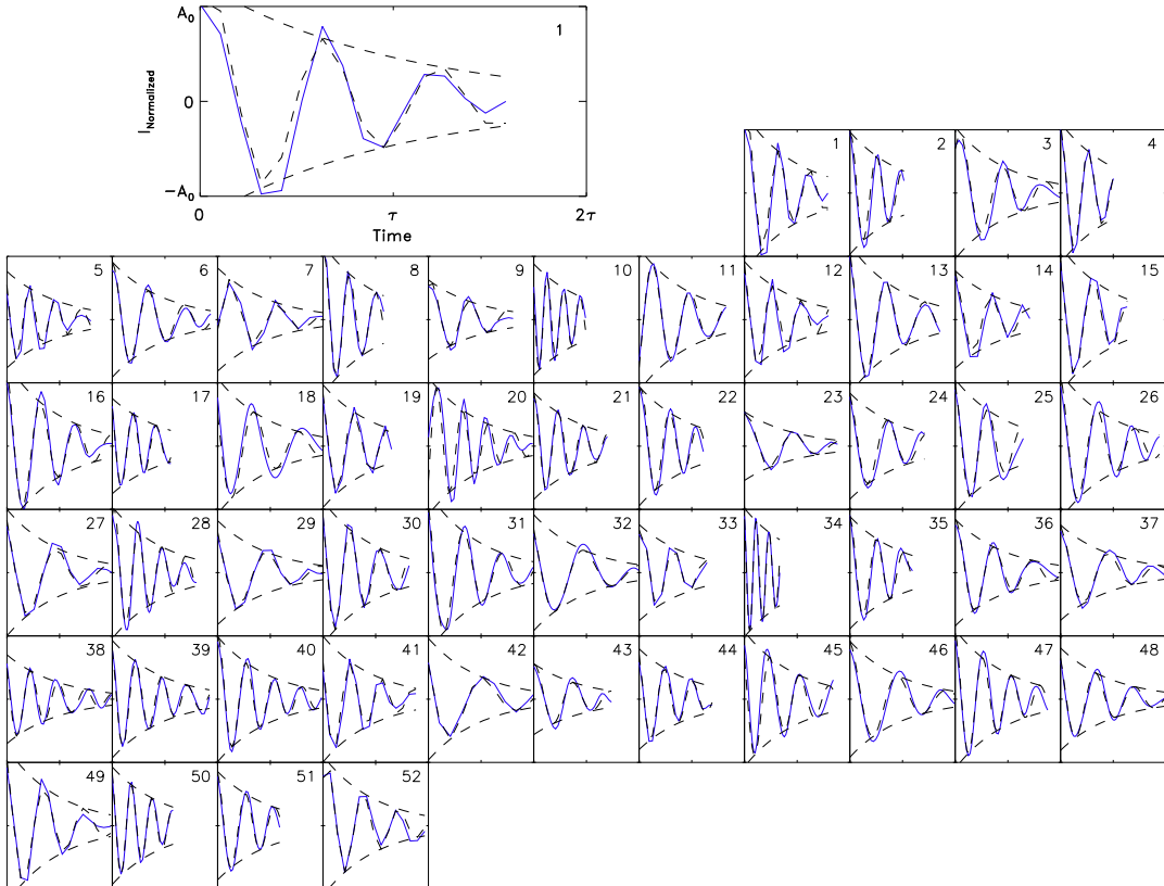
Fig. 6.— QPPs in stellar flares (blue) and the best-fitting damped harmonic functions (dashed). For visualization, the scales of the horizontal and vertical axes are normalized to the maximum amplitudes of the exponential function and damping times, as shown in the zoomed plot for the first sample.
