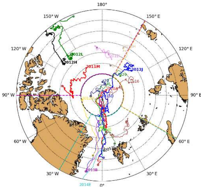
Figure 1. Drift trajectories of all selected buoys (IMBs and snow buoys) in 2010 to 2015. The symbol “★” indicates the start of the drift and “○” signals the end of the drift. Buoys are labelled at the beginning or the end of the drift using the same colour as trajectories. Buoys used for model simulations are highlighted with a solid thick line and bold font. Dashed thick lines illustrate our definition for sectors: central Arctic (black; north of 86° N), and south of 86° N: Pacific sector (magenta; 90° W–150° E), Atlantic sector (cyan; 30° W–60° E) and Laptev Sea (orange; 60–150° E) used in Fig. 6.
