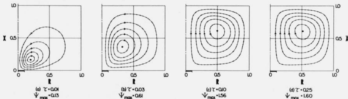
FIGURE 2. Transient streamline fields calculated with method V at various times ( \tau ), Gr = 1 \times 10^5 .
