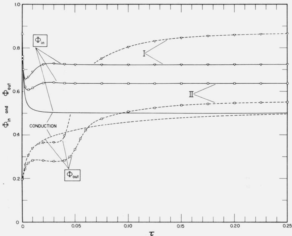
FIGURE 7. Dimensionless heat flow into ( \Phi_{in} ) and out of ( \Phi_{out} ) the enclosure as a function of time ( \tau ) for methods I and II ( Gr=1 \times 10^6 ) and static conduction (all methods).
