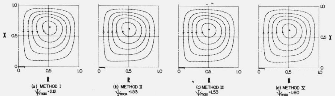
FIGURE 4. Steady-state streamline fields for the various numerical methods, Gr = 1 \times 10^5 .
