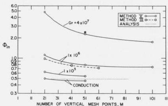
FIGURE 10. Steady state dimensionless heat flow ( \Phi_{in} ) versus number of vertical mesh points ( M ). Number of radial mesh points ( N ) held fixed at N = 21 (except for one solid data point for which N = 31 ).
