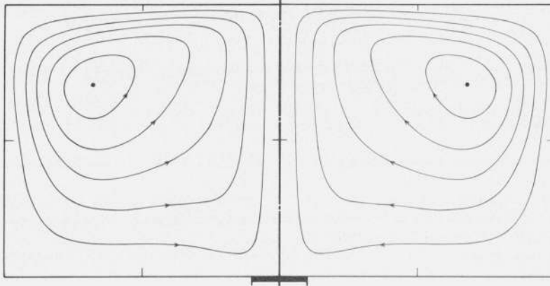
FIGURE 11. Comparison of numerical results of method V (from reference [18]) with physical experiment (from reference [17]) at Gr = 4 \times 10^6 .
