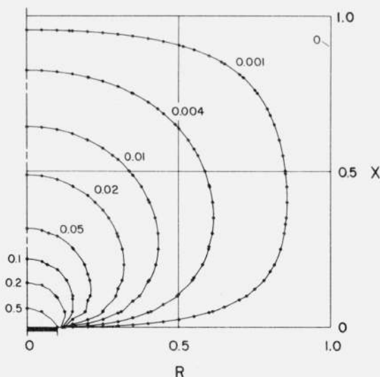
FIGURE 6. Static conduction temperature field at steady state, all methods. Temperature ( \theta ) is the curve parameter; the heat source (thick line on floor) is at \theta = 1 .
