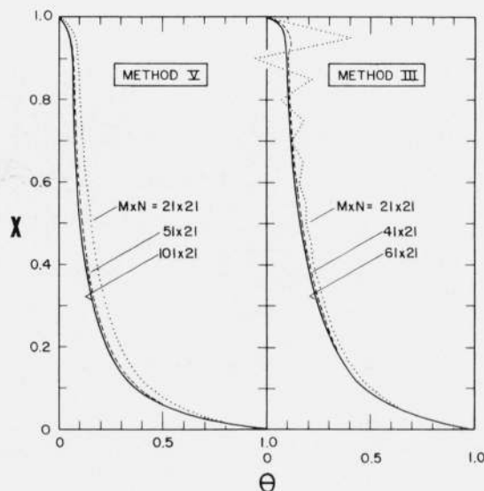
FIGURE 9. Steady state distribution of temperature ( \Theta ) with height ( X ) along the centerline; methods III and V, Gr = 1 \times 10^6 . Curve parameter is the number of vertical mesh points ( M ).
