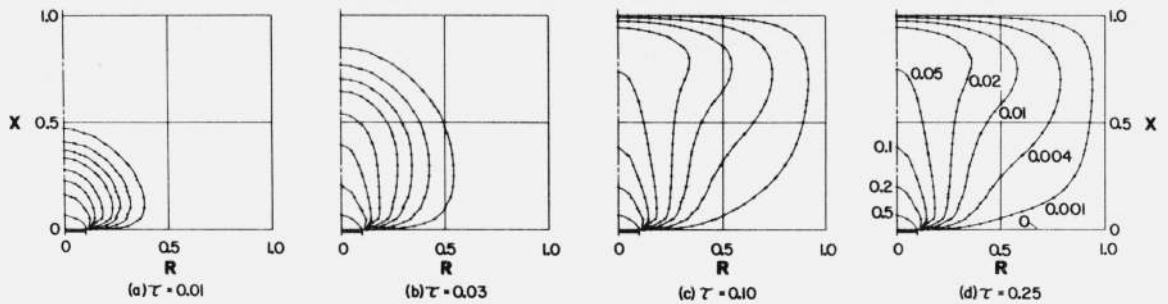
FIGURE 3. Transient temperature fields calculated with method V at various times ( \tau ), Gr = 1 \times 10^5 .
