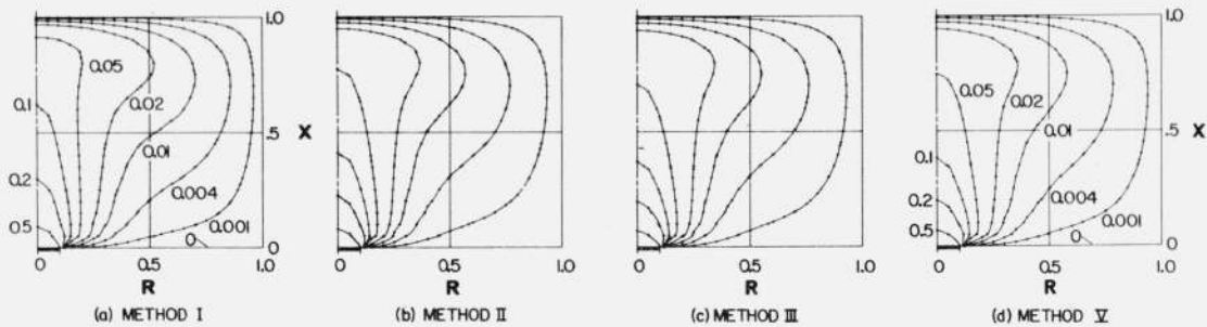
FIGURE 5. Steady state temperature fields for the various numerical methods, Gr = 1 \times 10^5 . Results for methods III and IV are identical. Temperature ( \theta ) is the curve parameter; the heat source (thick line on floor) is at \theta = 1 .
