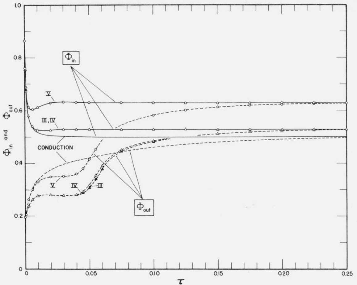
FIGURE 8. Dimensionless heat flow into ( \Phi_{in} ) and out of ( \Phi_{out} ) the enclosure as a function of time ( \tau ) for methods III, IV and V ( Gr=1 \times 10^5 ) and static conduction (all methods).
