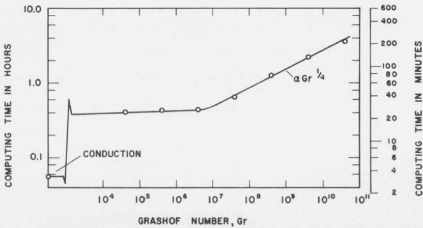
FIGURE 12. Computing time required for method V at several Grashof numbers ( Gr ), numerical study of reference [18]. Calculations carried from quiescent initial conditions to steady state with a M \times N = 51 \times 21 grid.
