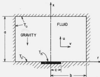
FIGURE 1. Cylindrical enclosure and coordinate system.
