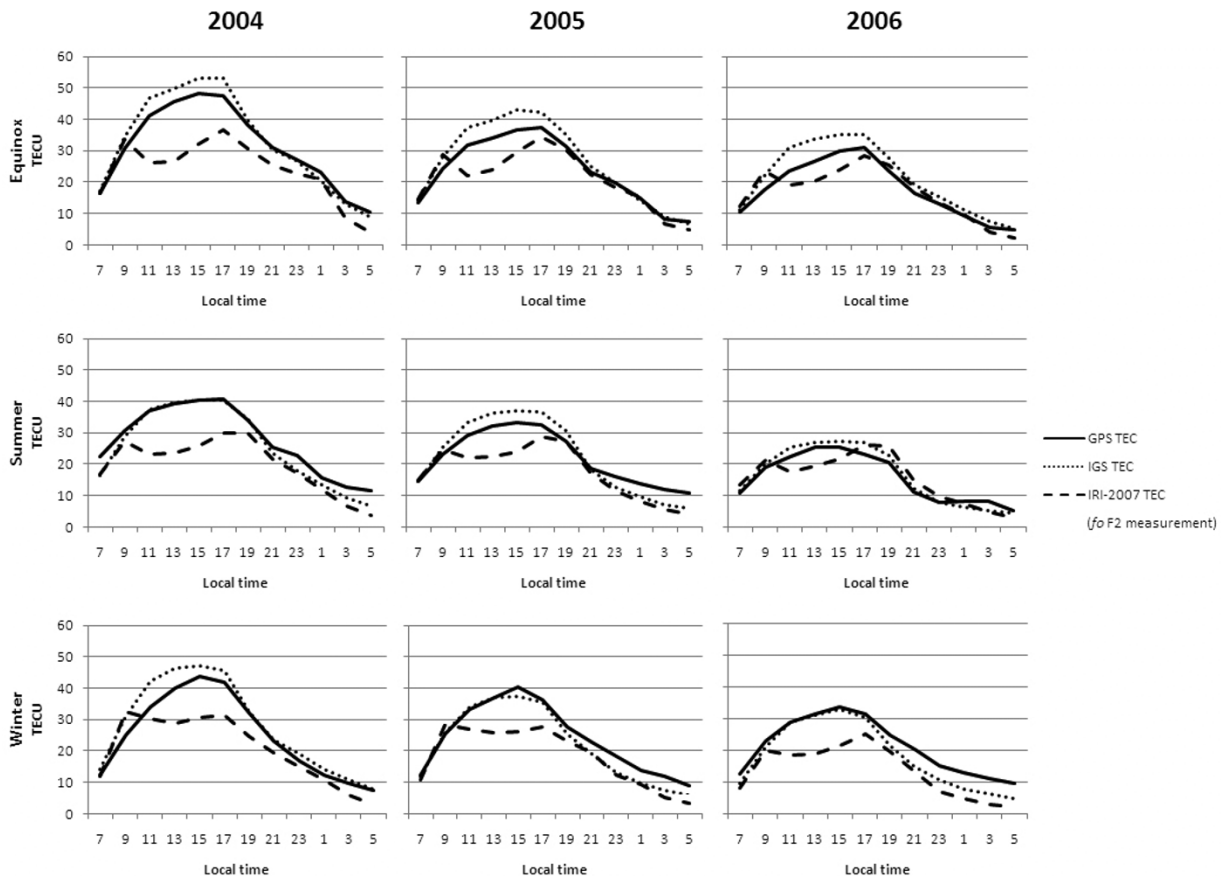
Fig. 2. Seasonal median values of GPS TEC, IGS TEC and IRI-2007 TEC at a Chumpon station for the three seasons, namely, equinox, summer and winter, respectively, during the period 2004–2006.
