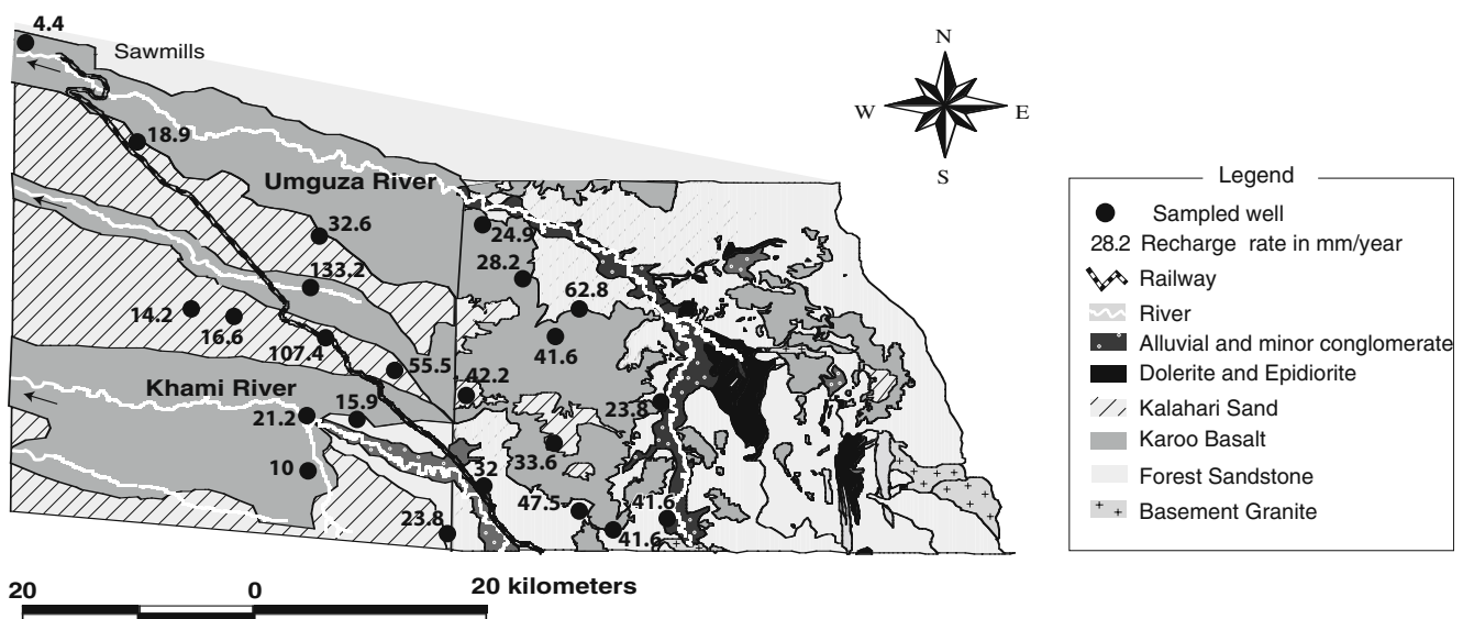
Fig. 4 Recharge determined with the chloride mass balance method
