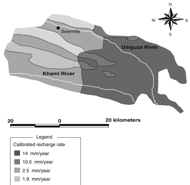
Fig. 10 Calibrated recharge rates; case with no transpiration from the groundwater system
