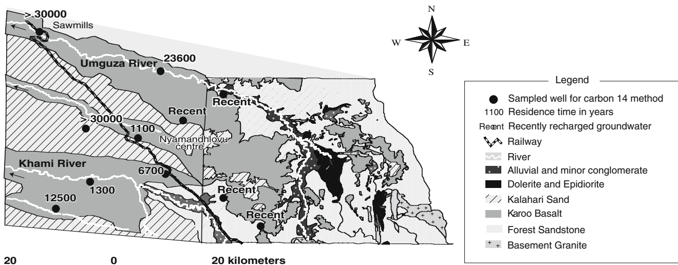
Fig. 8 Groundwater ages determined with the 14 C method
