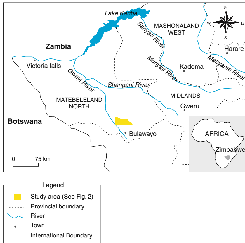
Fig. 1 Location map of study area in Zimbabwe
