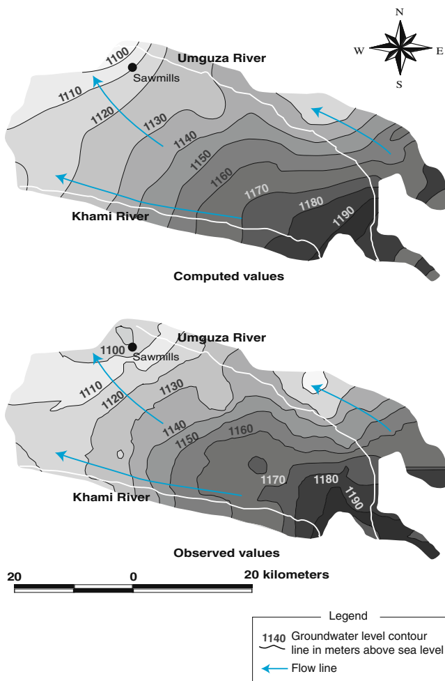
Fig. 9 Groundwater levels for the Forest Sandstone aquifer
