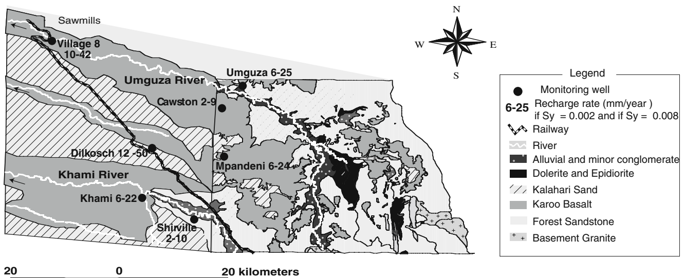
Fig. 6 Recharge determined with the water-table fluctuation method
