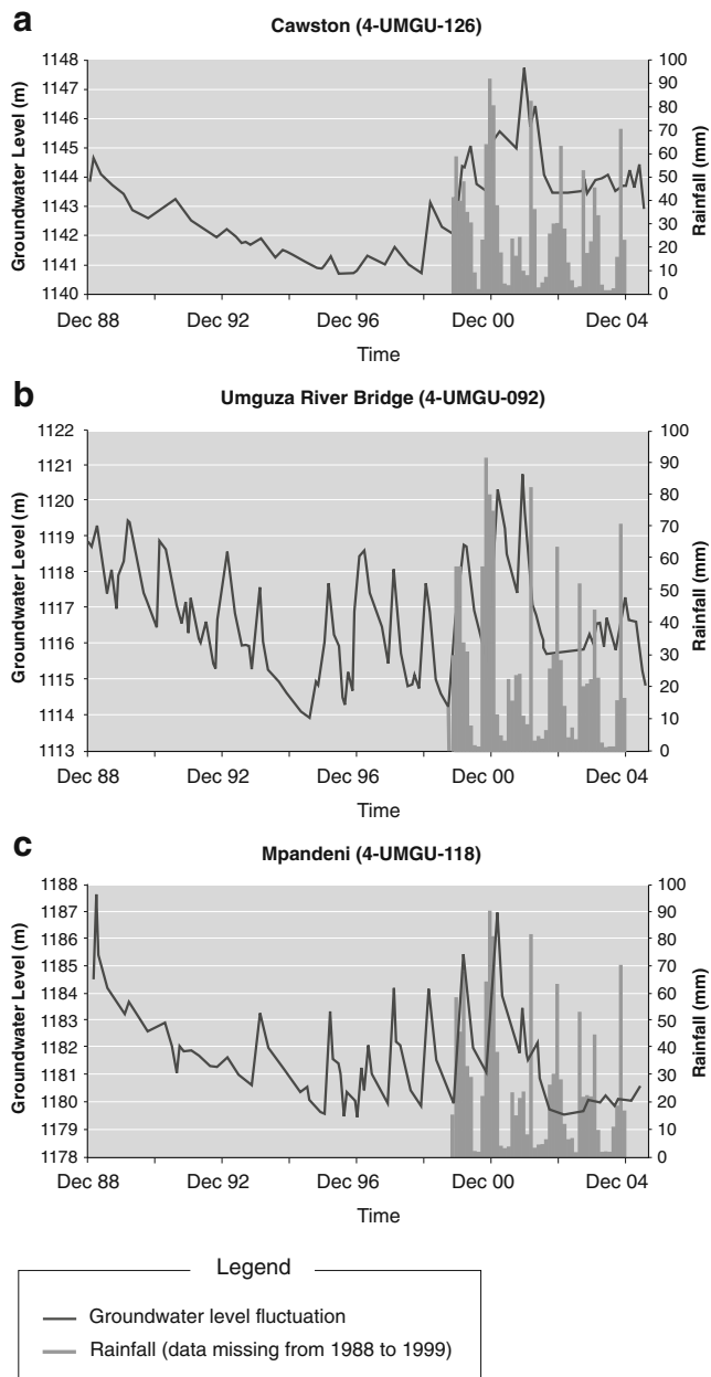
Fig. 5 Precipitation–groundwater level relationships
