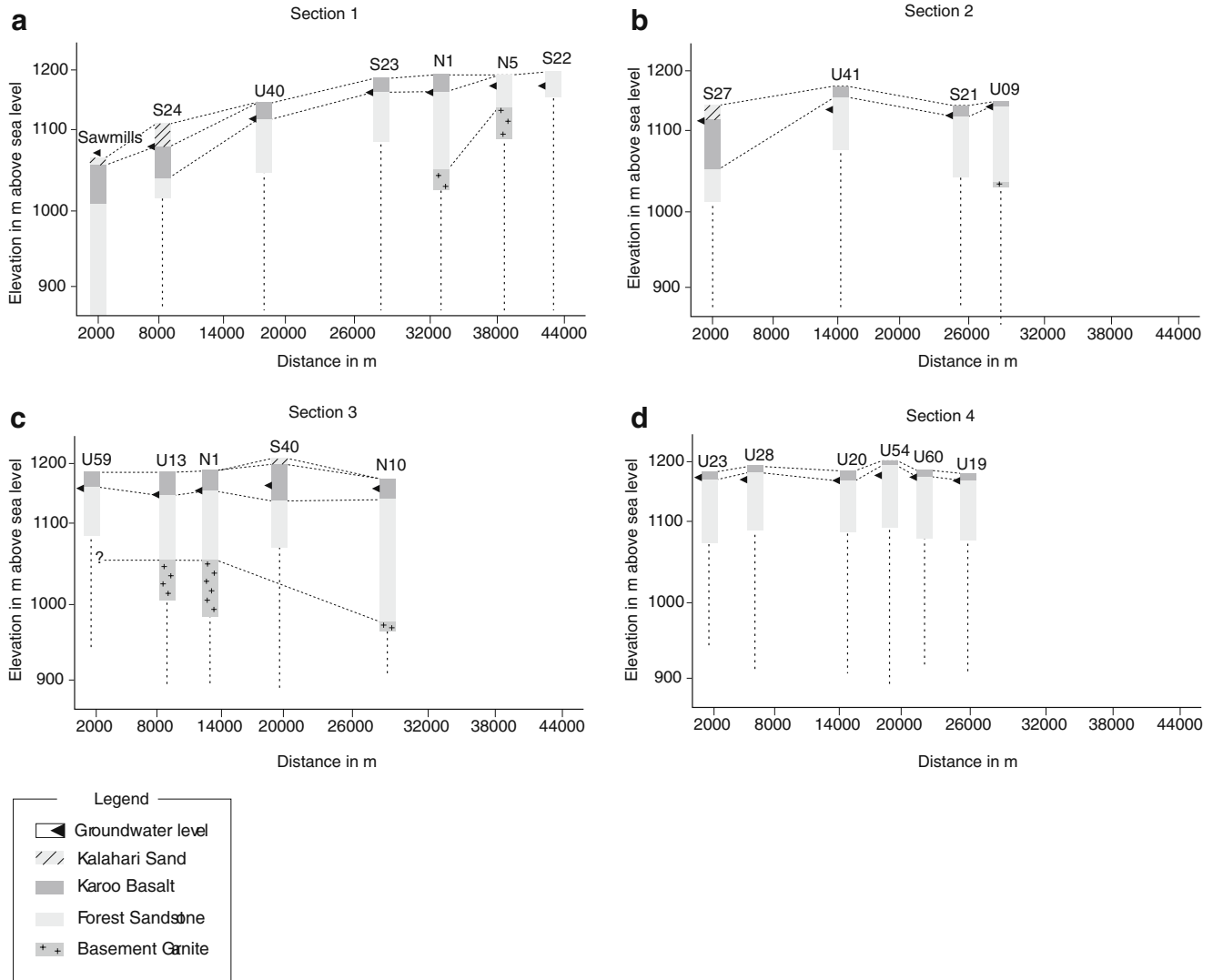
Fig. 3 Cross sections (see Fig. 2 for locations)
