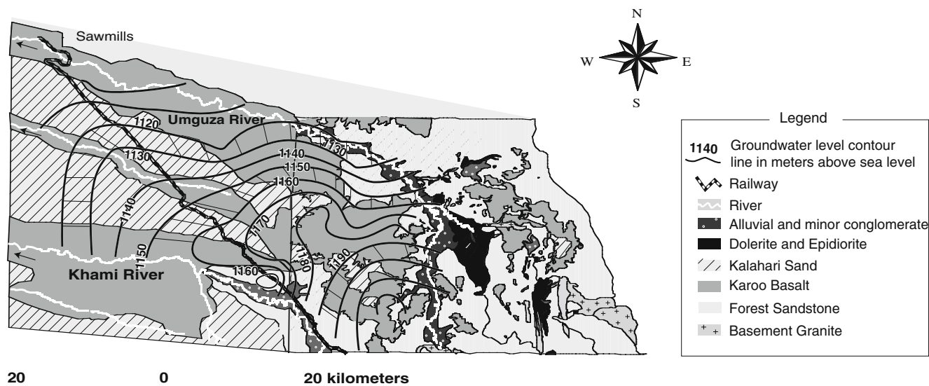
Fig. 7 Groundwater level contour map and flownet computation method
