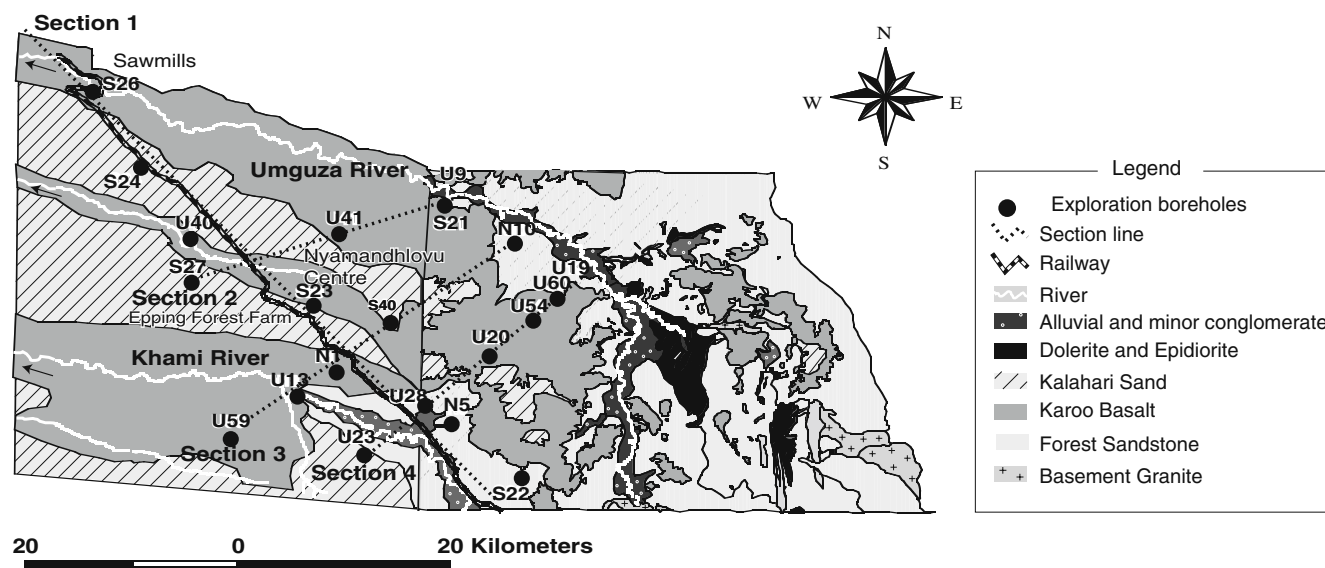
Fig. 2 Geology of the area showing traverses of cross sections
