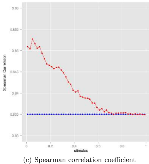
Figure 7. Obtained results for the three commonly used correlation coefficient: Pearson, Kendall and Spearman. The red line and the blue line respectively represent the computed correlation coefficient between MLDS and the original MS-SSIM values and between MLDS and weighted MS-SSIM.
