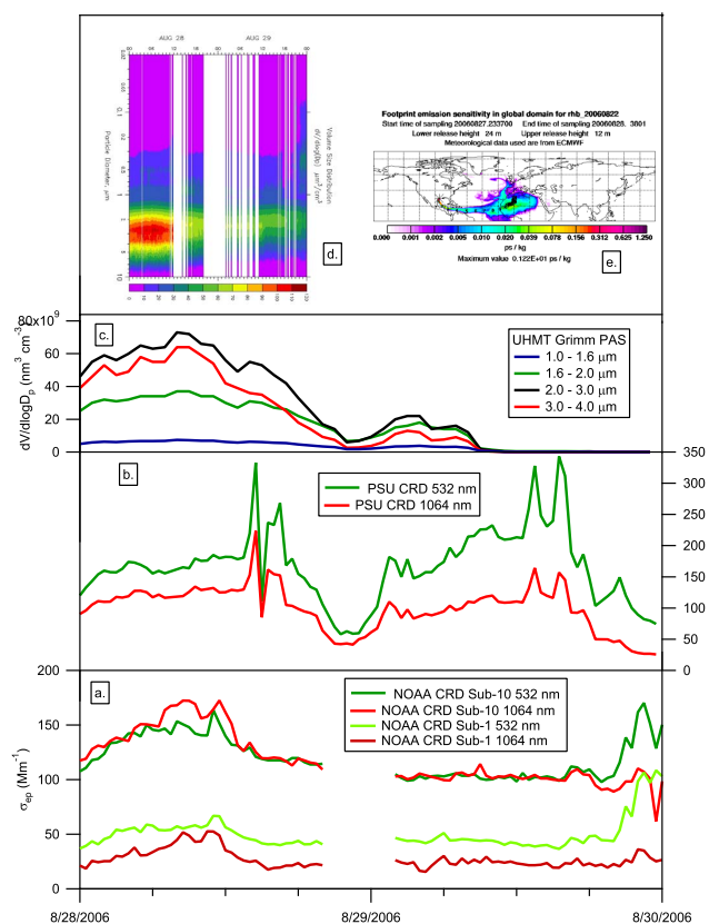
Fig. 2. Time series for the period 28 August–30 August 2006 of: panel (a) NOAA CRD sub 1 and sub 10 \mu\text{m} , 85% RH, 532 and 1064 nm \sigma_{\text{ep}} ; panel (b) PSU CRD 532 and 1064 nm \sigma_{\text{ep}} ; panel (c) 1 to 4 \mu\text{m} , size bins of the PAS at the UHMT site; panel (d) volume concentration size distribution from the DMPS/APS on the RHB; and (e) FLEXPART trajectory analysis showing transport patterns from the Saharan region to the Gulf of Mexico on 27 August.
