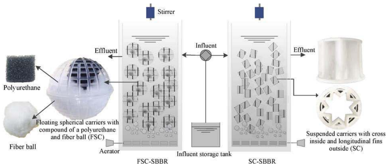
Fig. 1. Schematic diagram of the reactor.
