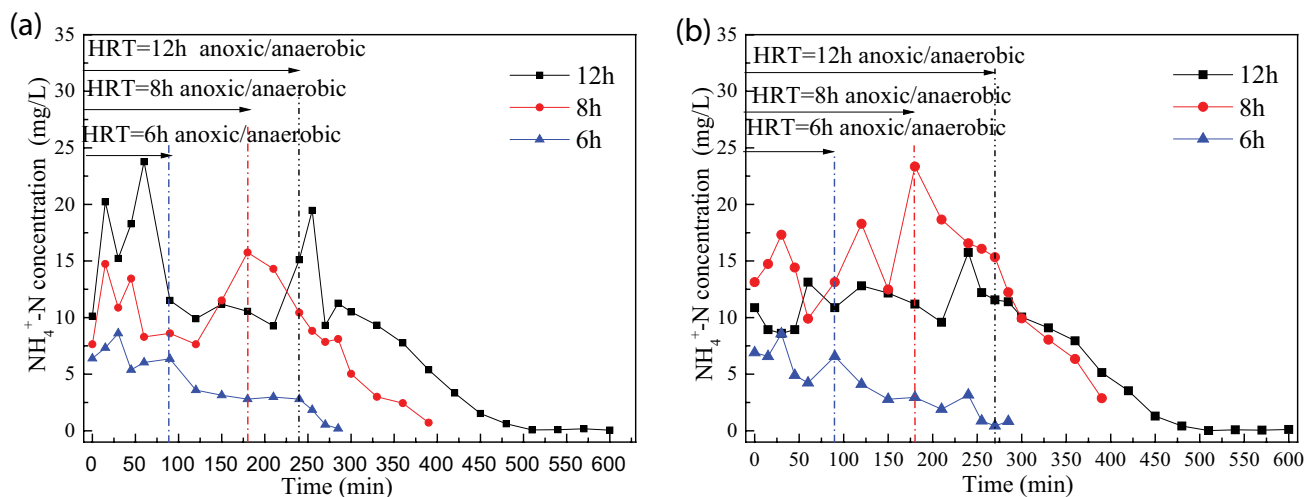
Fig. 8. Periodic variation of ammonia nitrogen contents in the supernatants of f_{sc} -SBBR and sc -SBBR at different HRTs.
