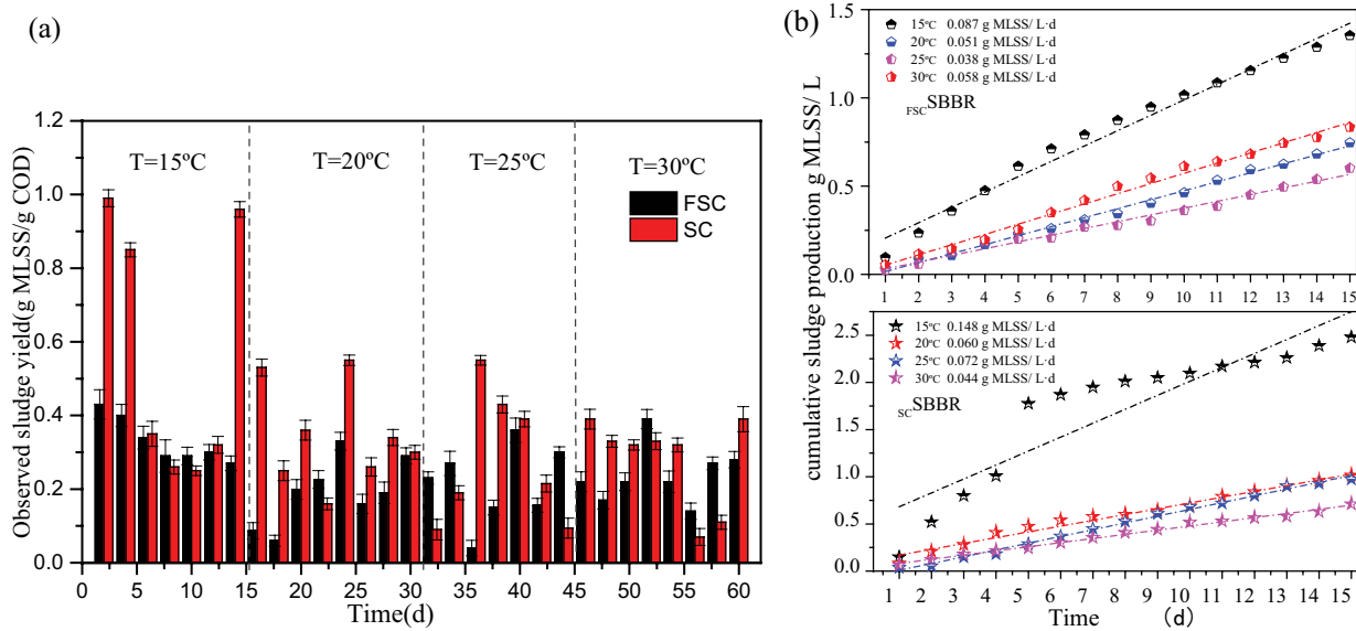
Fig. 2. Daily Y_{obs} (a) and cumulative sludge production and (b) of f_{sc} SBBR and s_c SBBR at different temperatures.
