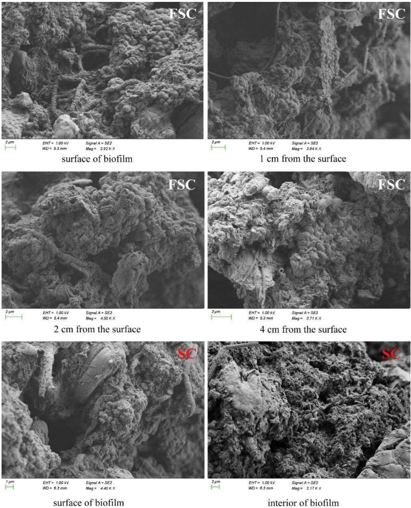
Fig. 9. SEM of biofilms in different regions of (a) FSC SBBR and (b) SC SBBR (from the surface to the bottom of the carrier).
