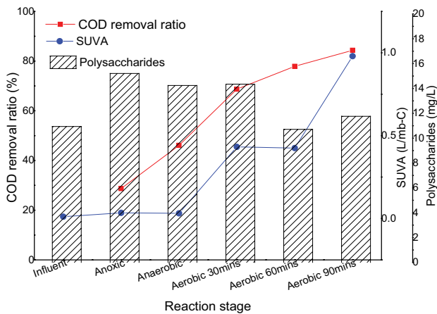
Fig. 10. Analysis of organic compounds in the supernatant of F_{SC} -SBBR samples at different stages of the system's operation cycle.
