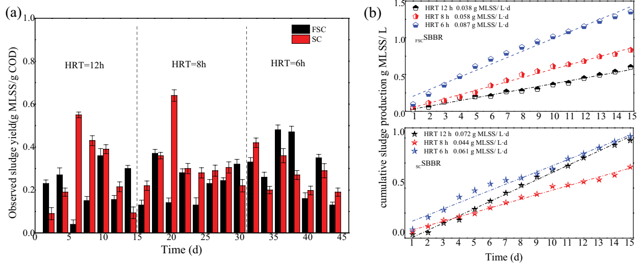
Fig. 7. Daily Y_{obs} (a) and cumulative sludge production (b) of f_{sc} -SBBR and sc -SBBR at different HRTs.
