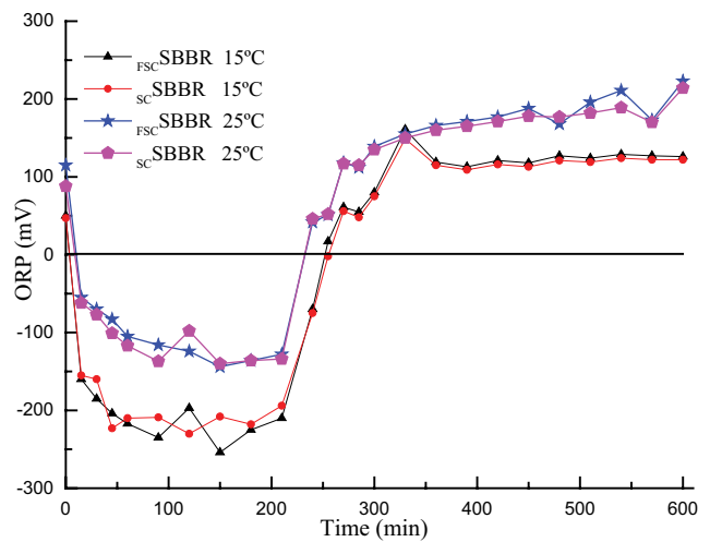
Fig. 3. Changes in ORP in f_{sc} SBBR and s_c SBBR at different temperatures.
