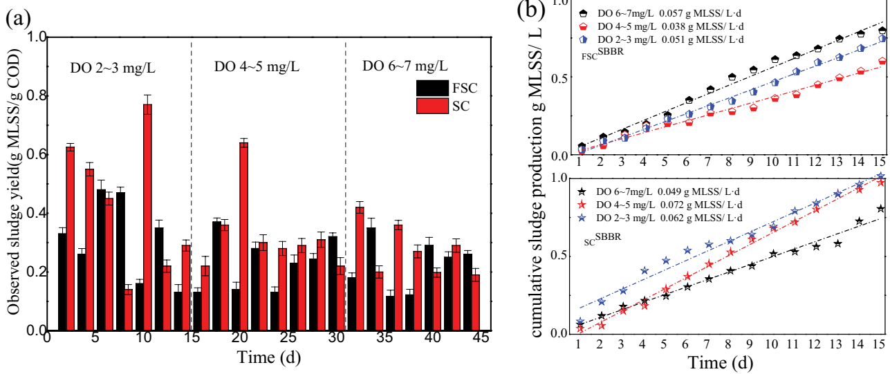
Fig. 5. Daily Y_{obs} (a) and cumulative sludge production (b) of f_{sc} -SBBR and s_{c} -SBBR at different DO concentrations.
