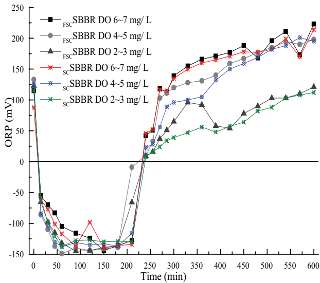
Fig. 6. Changes in ORP in f_{sc} -SBBR and s_{c} -SBBR under different DO conditions.
