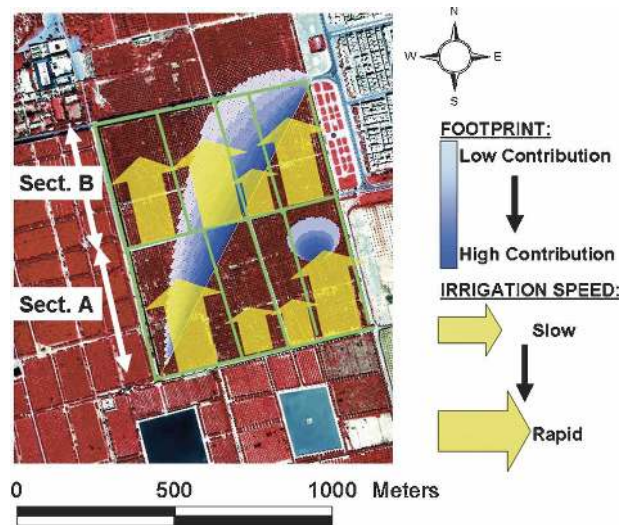
FIG. 4. Overview of irrigation schedule in the southern part of the Agdal olive yard. Irrigation starts in the southern sector A, simultaneously in all four zones (indicated with green lines), but advances with different speed in the different zones. Once sector A is fully irrigated, irrigation starts in sector B. Footprints of the LAS and EC system are shown in blue.
