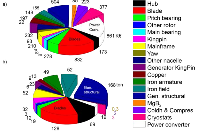
Fig. 3. 10 MW MgB 2 superconducting direct drive wind turbine rotor, generator and nacelles component cost and weight breakdown. a) Component cost in [k€] and b) component weight in [ton] according to the components outlined in [12]. The components associated with the superconducting drive train have been displaced from the center.
