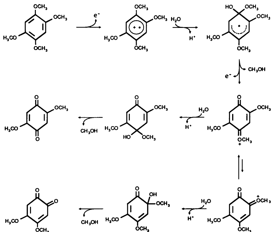
Scheme 1. Hypothetical scheme for the oxidation of 1,2,4,5-tetramethoxybenzene by lignin peroxidase/ H_2O_2 , HRP/ H_2O_2 or laccase/ O_2
