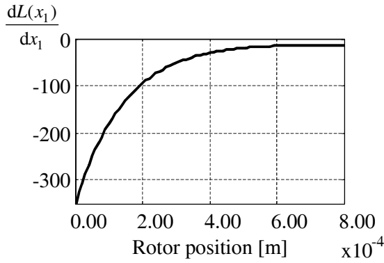
Fig. 9. Coil inductance vs. the rotor position.
