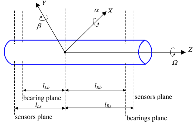
Fig. 12. Full model of the rotor.
