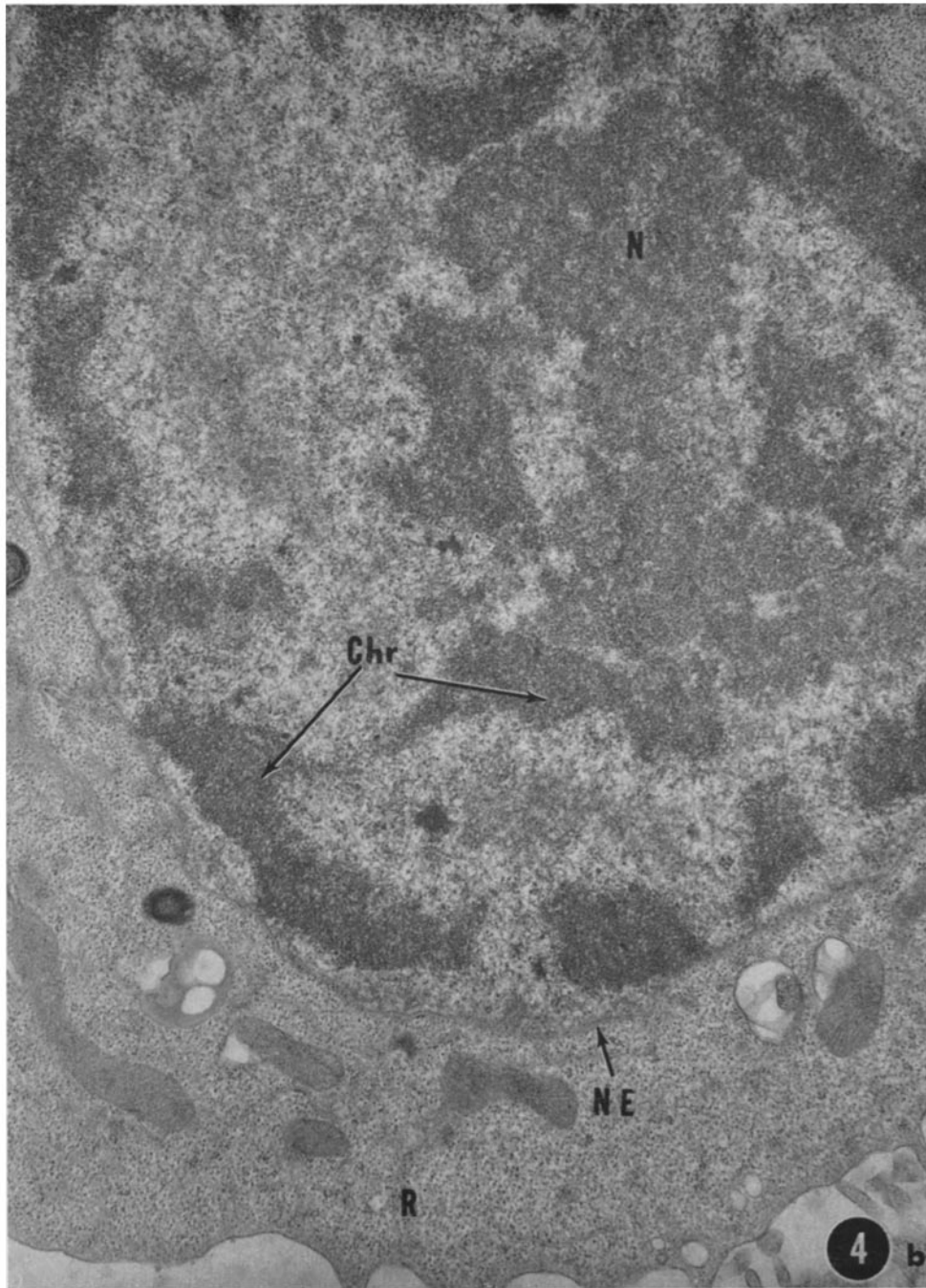
FIGURE 4 b Interphase cell treated for 10 min with 2.8 \times isotonic medium followed by isotonic medium for 10 min. The nuclear envelope is again visible and intact. The nucleolus has regained its fibrous component. This, in conjunction with the decodensing chromatin, gives the nucleus a telophase-like appearance. Few polyribosomes are seen. \times 13,000 .
