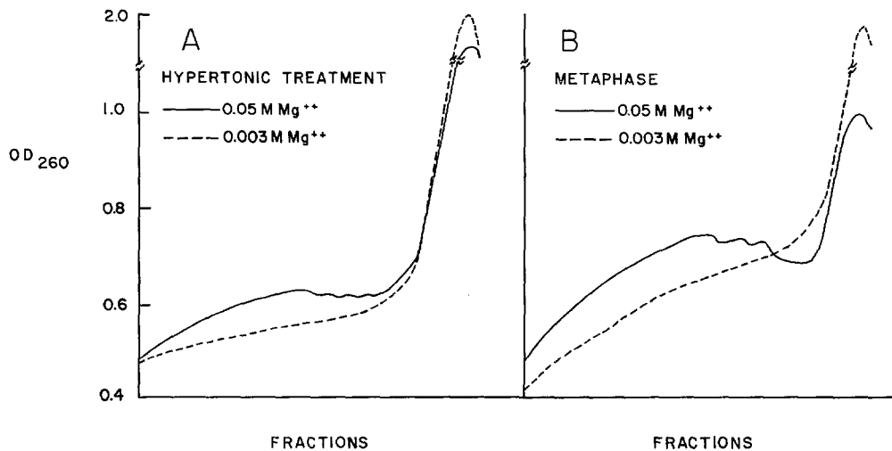
FIGURE 10 A Effects of 0.05 M Mg ++ on polyribosome breakdown following hypertonic treatment. 10 7 cells were incubated for 1 hr in isotonic medium containing either 0.003 M Mg ++ (---) or 0.05 M Mg ++ (—). Both samples were then resuspended in 1.6 × isotonic medium for 10 min, and polyribosomes were prepared and analyzed on sucrose gradients as in Fig. 8.
