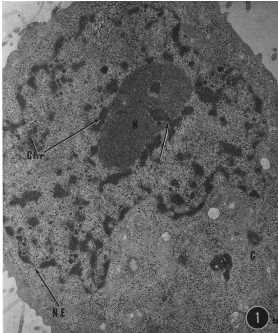
FIGURE 1 b Interphase cell treated for 2 min with 1.6 \times isotonic medium. Chromatin is condensed preferentially along inner aspect of nuclear envelope and about nucleolus. Nuclear envelope is ruffled. Nucleolus shows diffuse granularity and absence of fibrous component. Polyribosomes are intact. At arrow, the condensed intranucleolar chromatin is continuous with the chromatin in the nucleoplasm proper. \times 10,000 .
