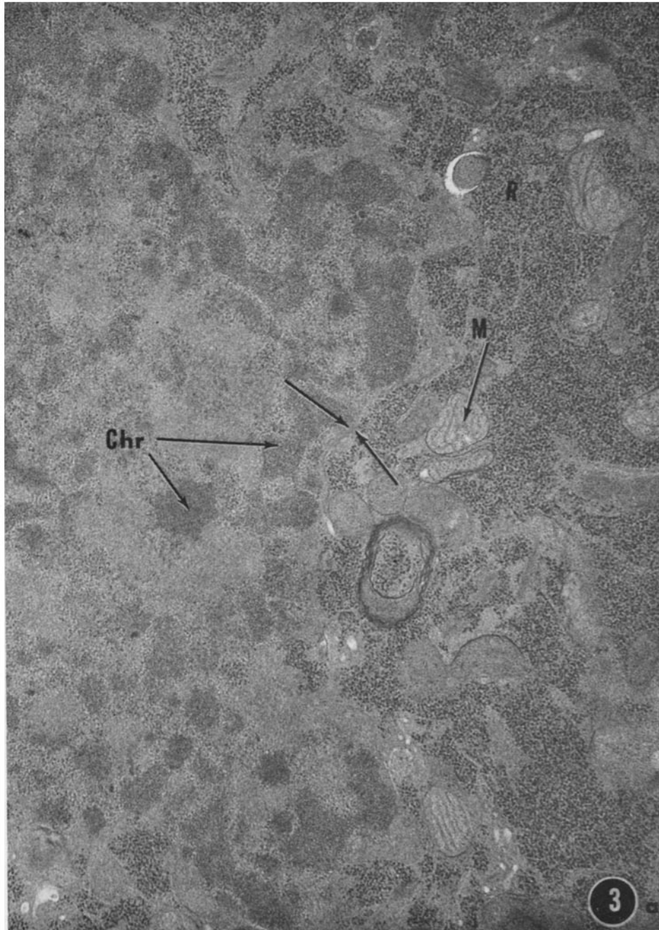
FIGURE 3 a Interphase cell treated for 10 min with 2.8 \times isotonic medium. Nuclear envelope is not visible along most of nuclear-cytoplasmic boundary. Mitochondrial and lysosomal membranes remain discernible although higher magnification (Fig. 3 b ) indicates that they too are affected by the high salt. Paired arrows indicate nuclear-cytoplasmic boundary. 3 a , \times 14,000; 3 b , \times 56,000.
