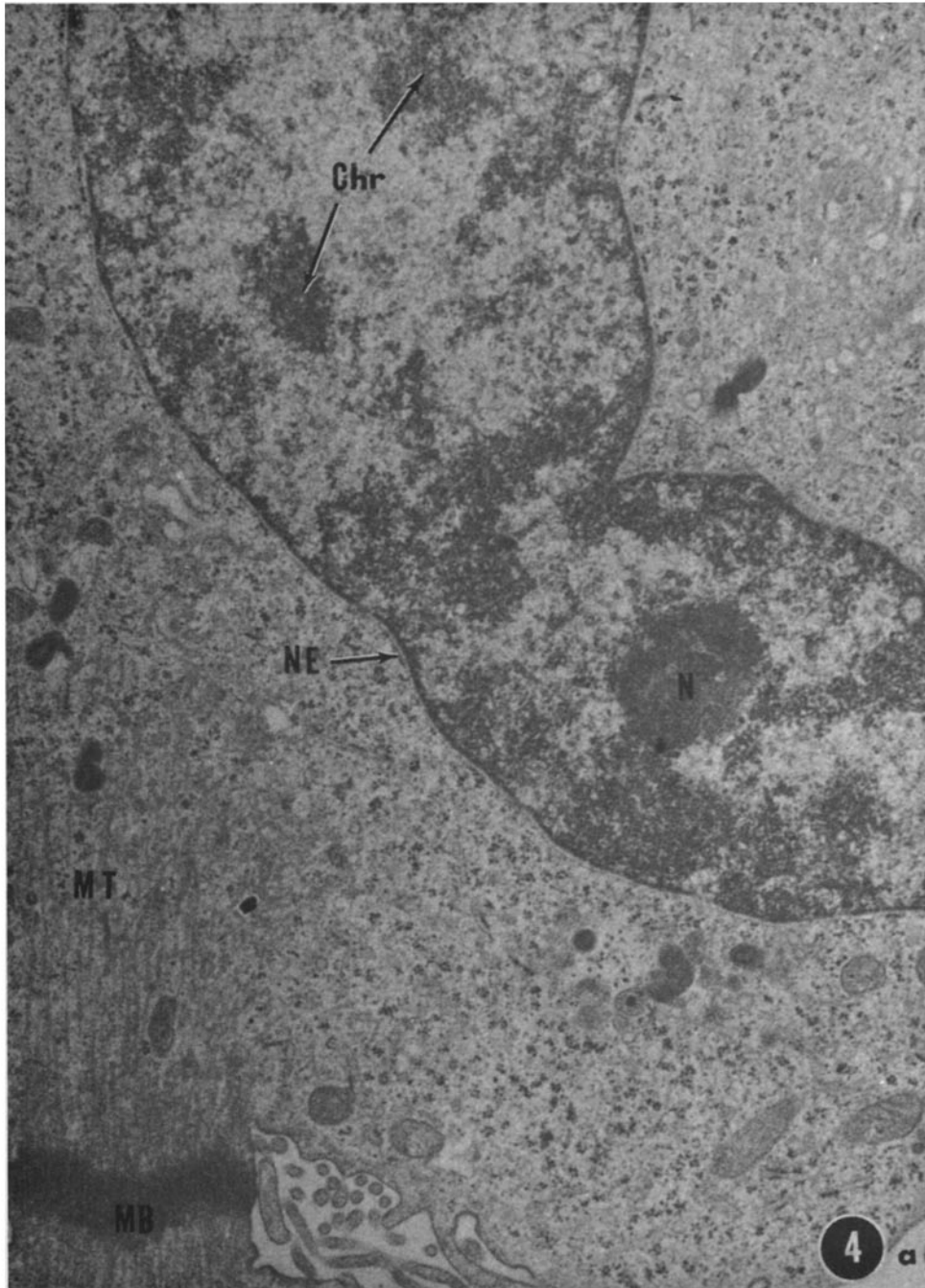
FIGURE 4 a Untreated telophase cell. \times 27,000 .
