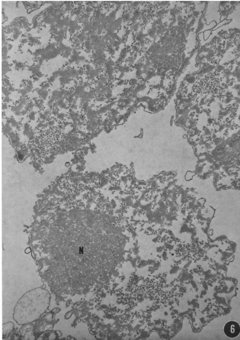
FIGURE 6 Electron micrograph of nuclei isolated in hypotonic Tris buffer and then exposed to 0.1 M \text{CaCl}_2 . Chromatin is grossly precipitated. \times 17,000 .
