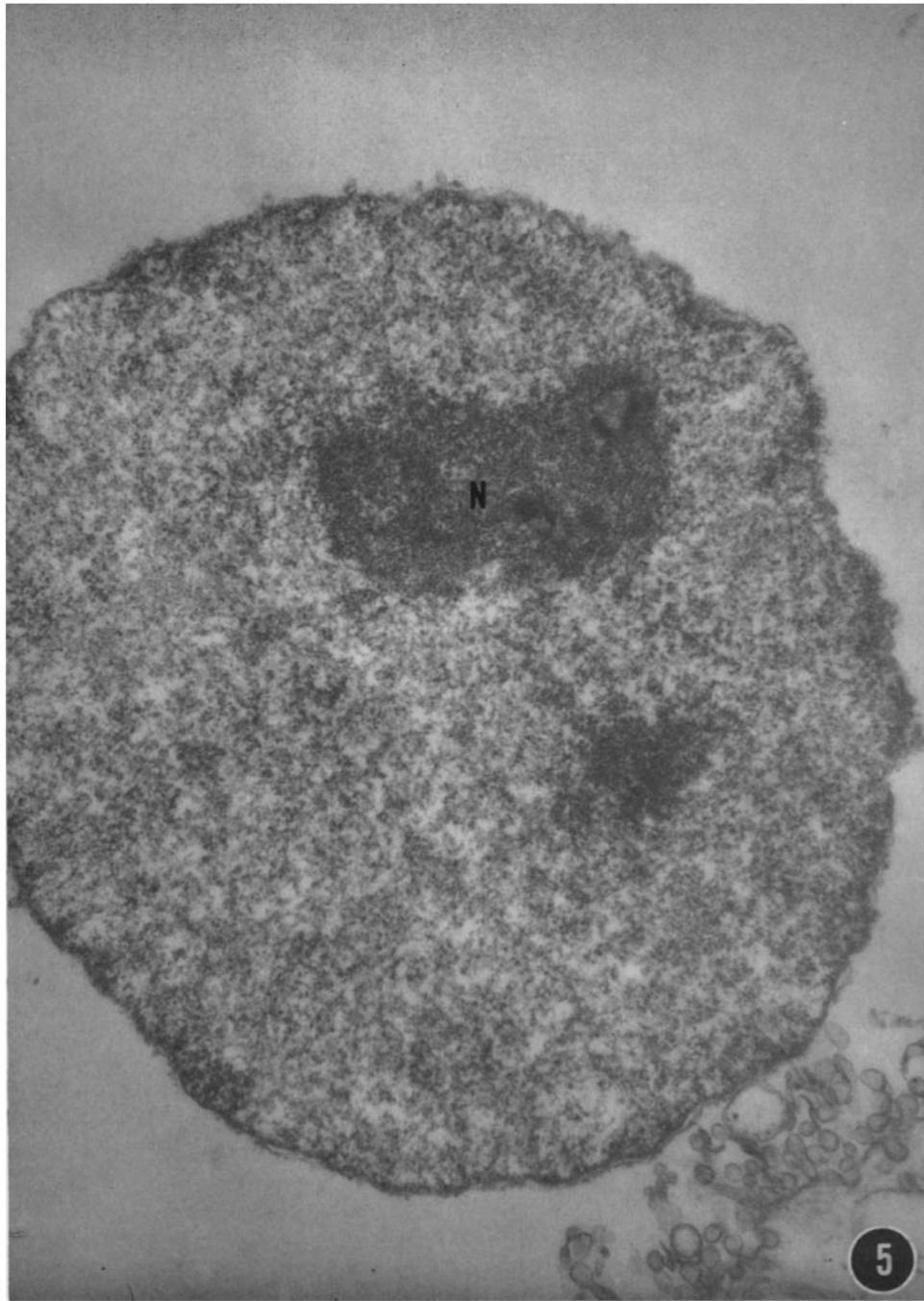
FIGURE 5 Electron micrograph of nucleus isolated in hypotonic Tris buffer, and then exposed to 1.6 \times isotonic medium. Morphology is not significantly different from that of nucleus in untreated interphase cell. \times 11,000 .
