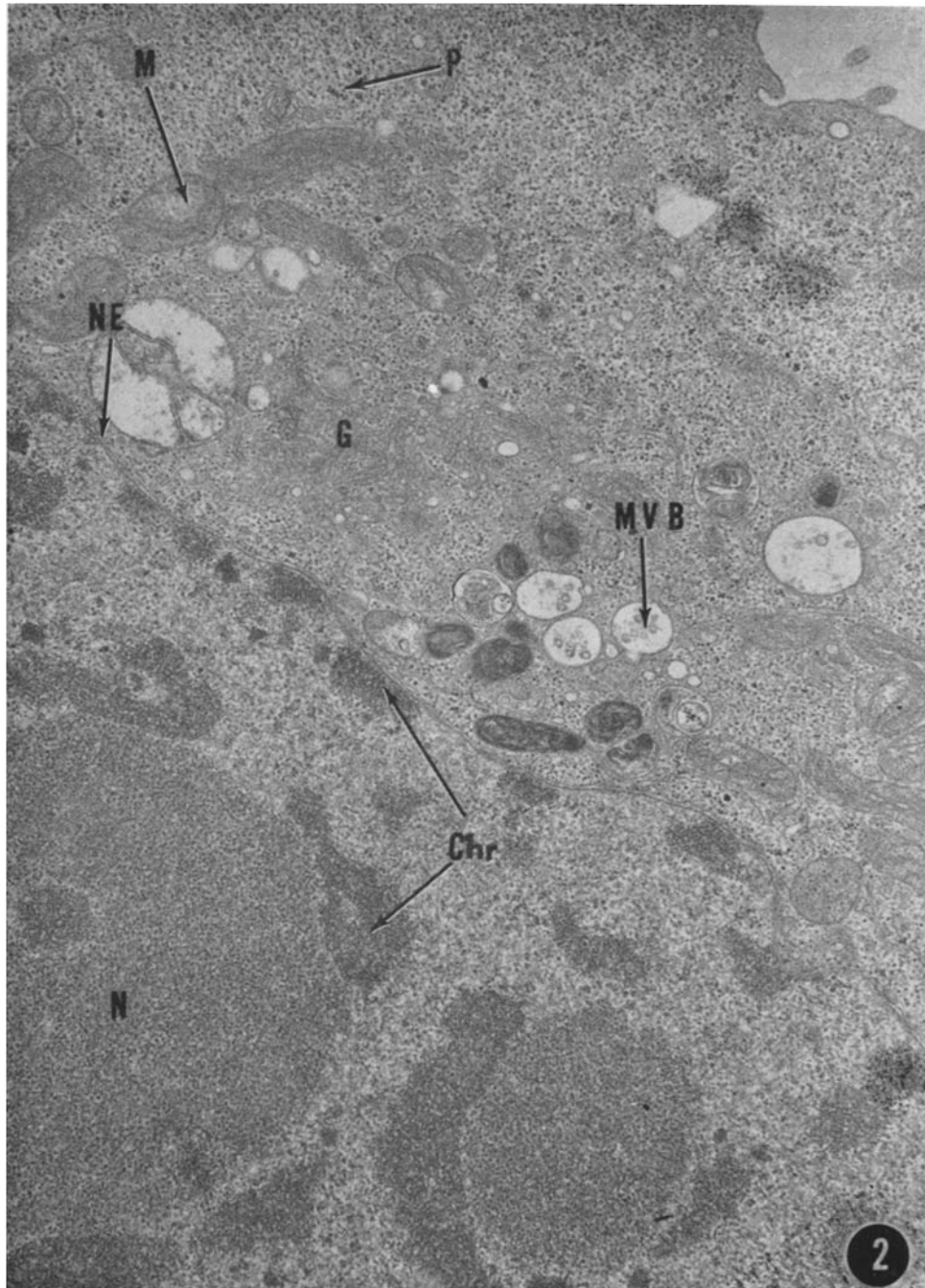
FIGURE 2 Interphase cell treated for 4 min with 1.6 \times isotonic medium. Cytoplasmic polyribosomes disaggregated. Other organelles show no further change. \times 16,000 .
