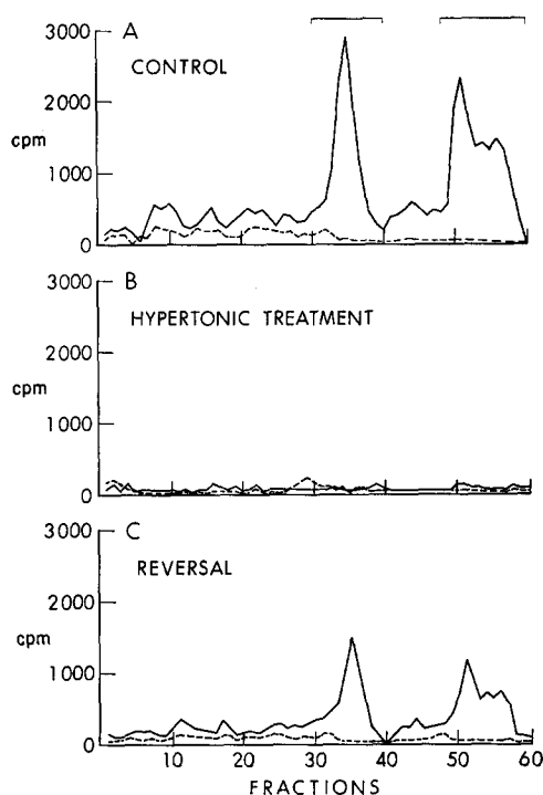
FIGURE 9 Effects of hypertonicity on histone synthesis. 2 \times 10^7 cells synchronized in S were: (A) labeled for 15 min with 5 \mu\text{C} of lysine- ^{14}\text{C} and 50 \mu\text{C} of tryptophan- ^3\text{H} , or (B) suspended in 2.8 \times isotonic medium for 10 min and then labeled, or (C) treated for 10 min with hypertonic medium and returned to isotonic medium containing label as in A. After washing and disruption by Dounce homogenization, the nucleohistones were extracted with 0.25 N HCl and analyzed by electrophoresis on polyacrylamide gels containing sodium dodecyl sulfate as described previously (15). The histones are bracketed. (—) lysine- ^{14}\text{C} , (---) tryptophan- ^3\text{H} .
