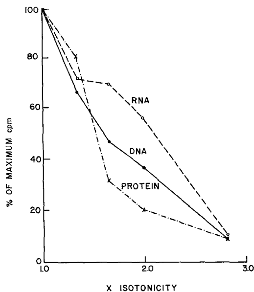
FIGURE 7 The effects of increasing tonicity on macromolecular synthesis. Aliquots of cells were made hypertonic by appropriate addition of NaCl and incubated for 10 min at 37^\circ C . Incorporation of DNA, RNA, and protein precursors into TCA-precipitable material was assayed as described in the text.
