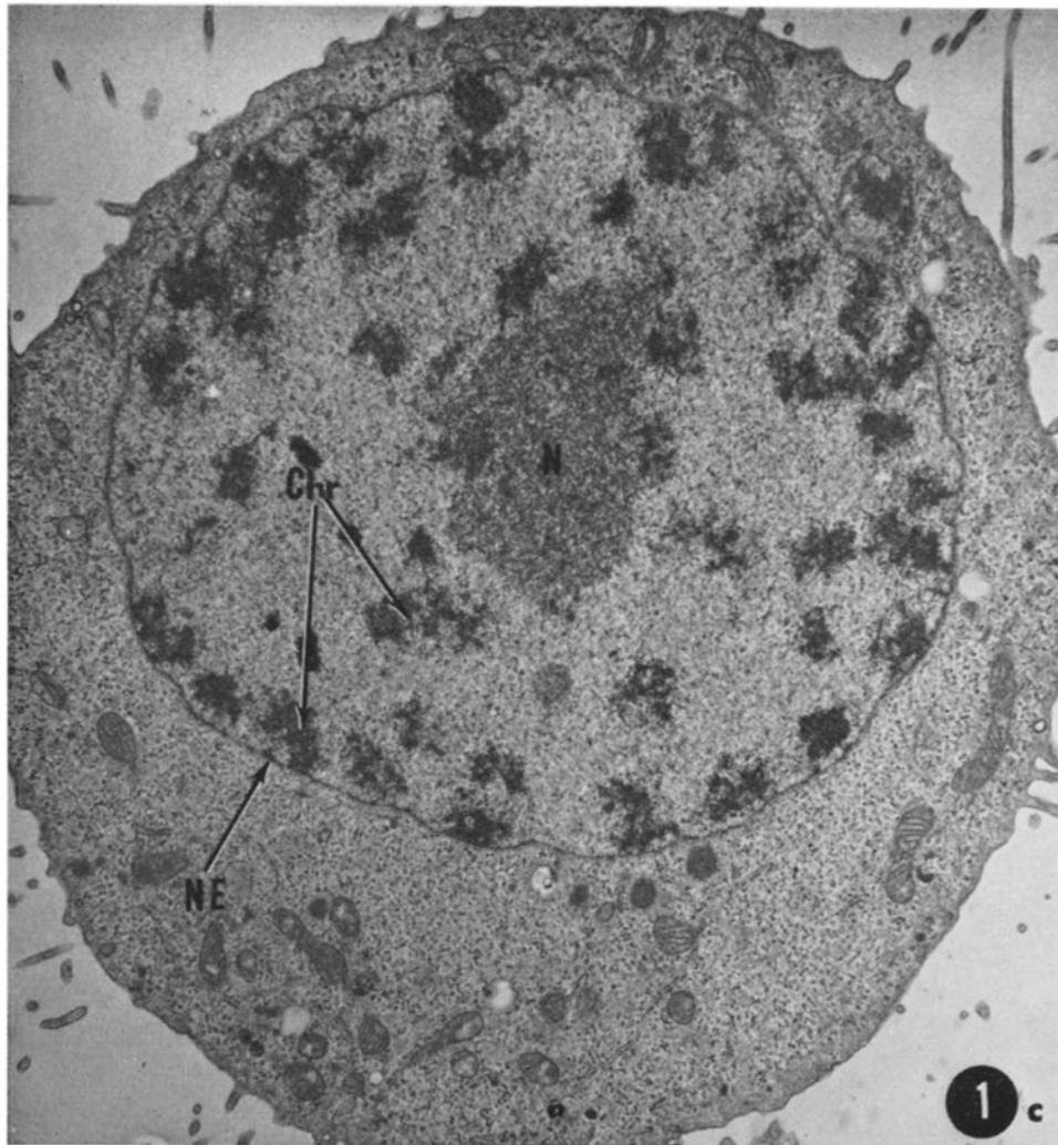
FIGURE 1 c Untreated prophase cell shown for comparison with Fig. 1 b . Distribution of condensed chromatin is similar; however, both chromatin and nucleolus display a more fibrous appearance than they do following hypertonic treatment. \times 7,000 .
