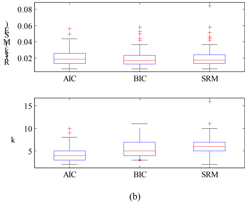
Figure 3: [Cherkassky] Comparison results for univariate regression using k -nearest neighbors. Training data: n=30 , noise level \sigma = 0.2 (a) sine squared target function (b) piecewise polynomial target function
