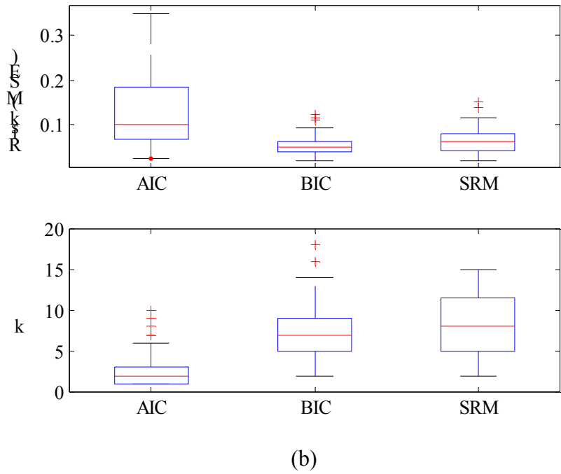
Figure 5: [Cherkassky] Comparisons results for two dimension sinc target function using k -nearest neighbors, sample size n=50 (a) \sigma =0.2 (b) \sigma =0.4
