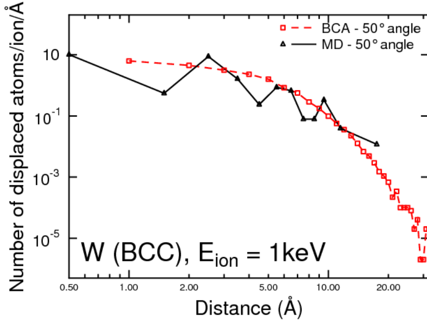
Figure 6: Atom displacement statistics for single 1 keV \text{Ar}^+ impact on crystalline W at 50^\circ incidence angle.
