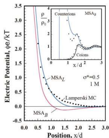
Figure 11. MSA_B and MSA_L implementation schemes compared with Lamperski MC electric potential and ion density profiles. MSA_B produces charge inversion in contrast to MSA_L and MC.
