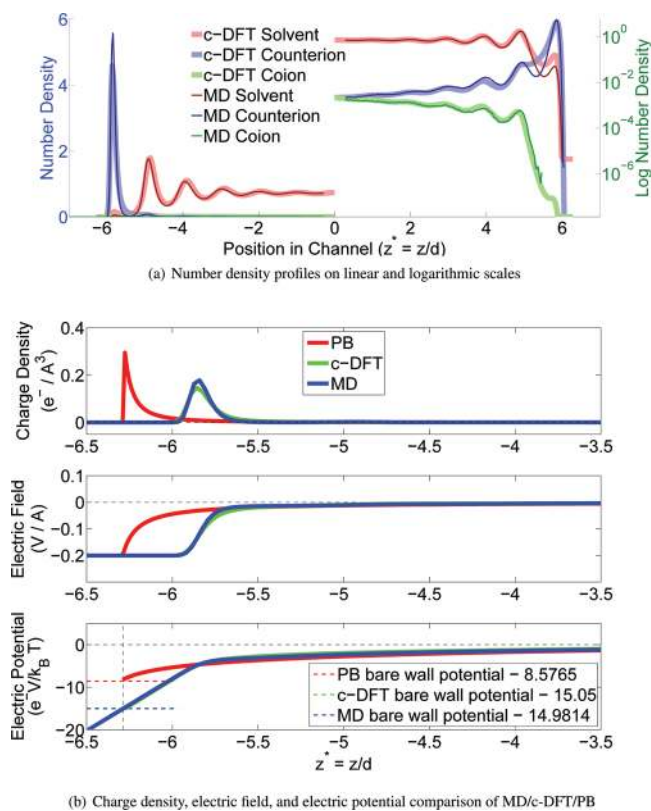
Figure 5. MD/c-DFT EDL comparison for 0.88 normalized surface charge. Electrolyte concentration is 113.45 mM (100 mM target). Bulk solvent density, normalized by d^3 , is 0.72227 (0.7 target).
