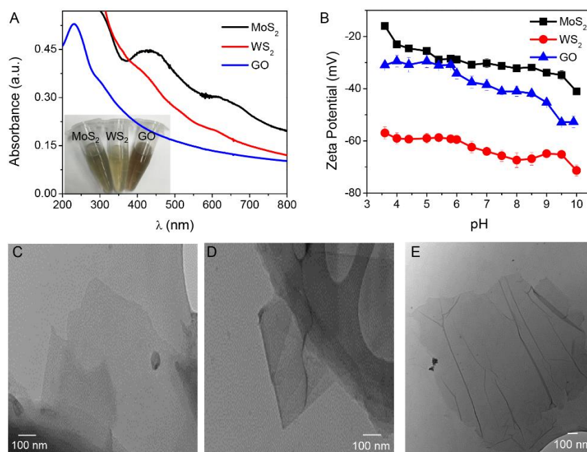
Figure 2. Characterization of these three 2D materials. (A) UV-vis spectra of MoS 2 and WS 2 (100 \mu\text{g/mL} ) and GO (25 \mu\text{g/mL} ) dispersed in water. Inset: a photograph of these materials (0.5 mg/mL each). (B) Zeta-potential of each material (0.05 mg/mL) as a function of pH in 10 mM buffer (acetate from pH 3.6 to 6; phosphate from pH 6 to 8.5; and carbonate from pH 9 to 10). TEM micrographs of (C) MoS 2 , (D) WS 2 and (E) GO.
