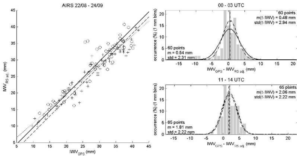
Figure 3: Comparison between IWW estimates obtained with GPS ( IWW_{GPS} ) and RS adjusted for the altitude difference ( IWW_{RS\ adj.} ).
