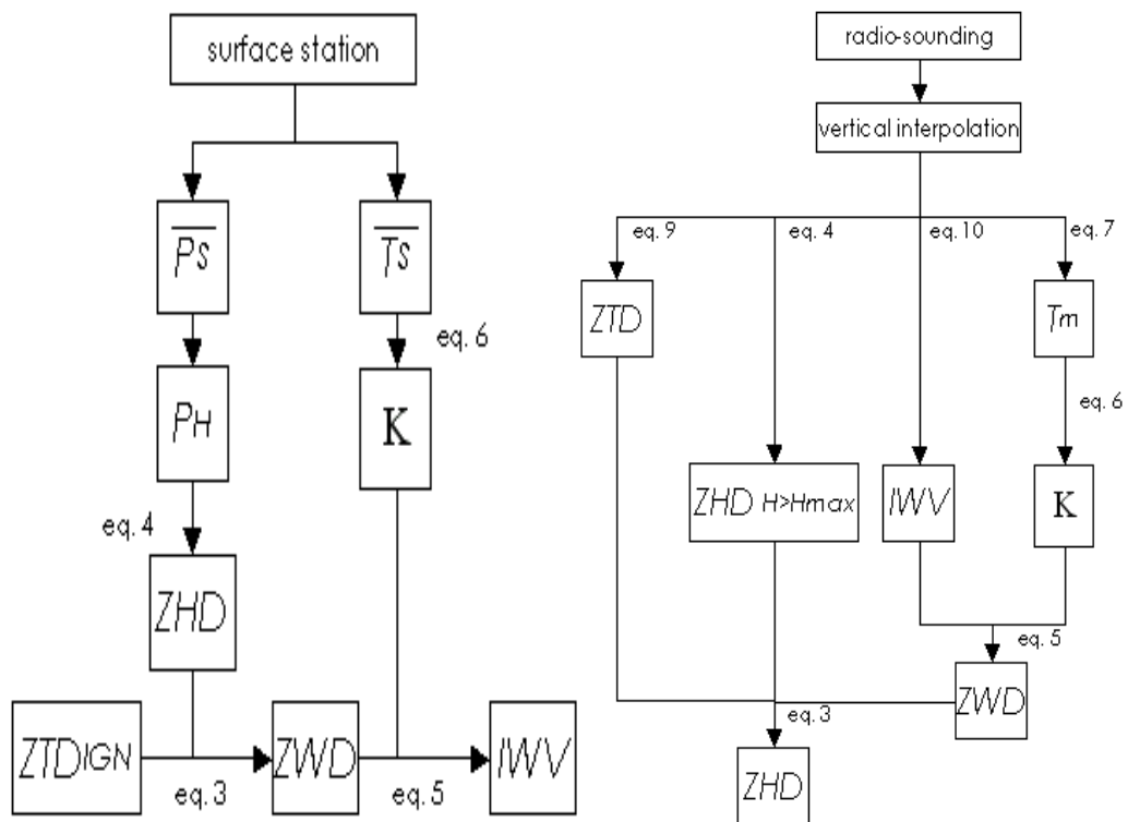
Figure 1: Flow charts of a) the GPS IZW calculation and b) the RS IZW estimate calculation.
