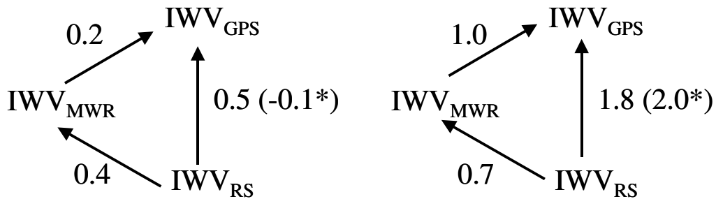
Figure 6: Nighttime and daytime summary of IWV estimates comparisons between GPS, RS, and MWR for the period of August 22 to September 24, 2002. (*)Note: between brackets the IWV difference between GPS and RS using all three months of common data for the period of August 19 to November 19, 2002.
