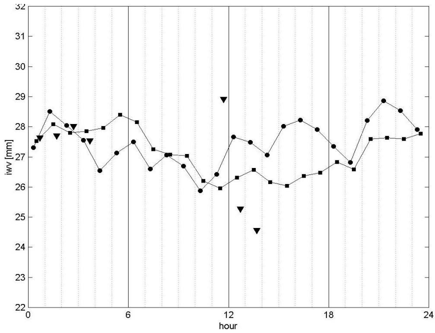
Figure 7: Diurnal variation of mean hourly IwV estimates obtained with GPS (circles), MWR (squares), and RS (triangles).
