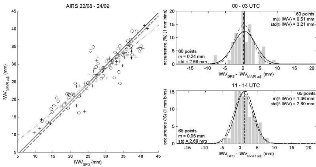
Figure 5: Comparison between IWV estimates obtained with GPS ( IWV_{GPS} ) and MWR adjusted for the altitude difference ( IWV_{MWR\ adj.} ).
