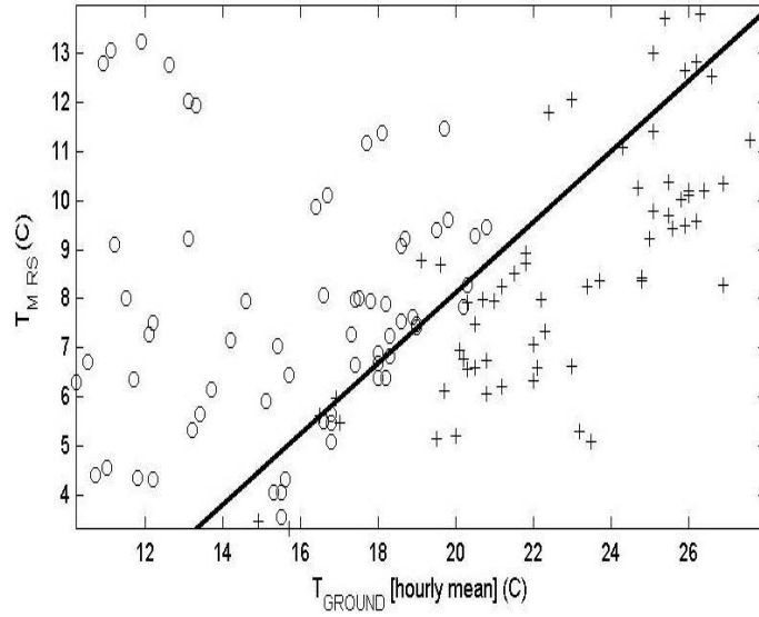
Figure 8: Comparison between T_m derived from RS (circles and crosses) and T_m estimated from surface temperature measurement using the relationship of equation (3) (bold straight line) as a function of the hourly mean surface temperature.
