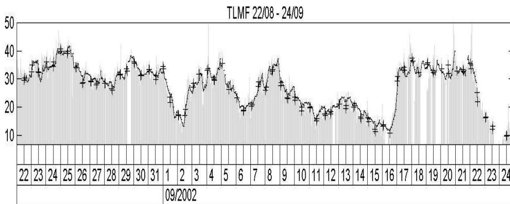
Figure 2: Time series of the IZW estimates retrieved with GPS (gray dashes), RS (crosses), and MWR (continuous black line) for the period August 22 to September 24, 2002.
