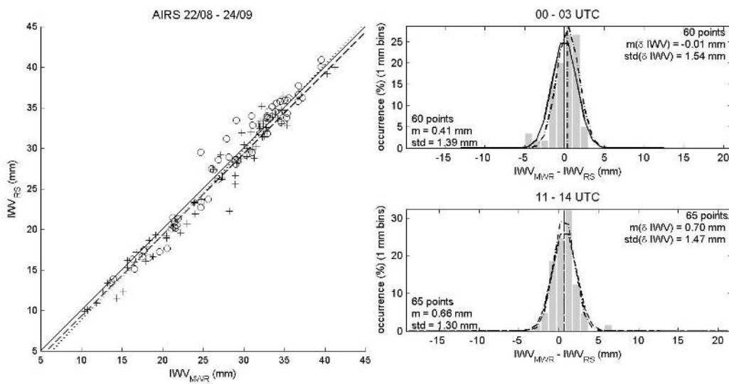
Figure 4: Comparison between IWW estimates obtained with MWR ( IWW_{MWR} ) and RS ( IWW_{RS} ).
