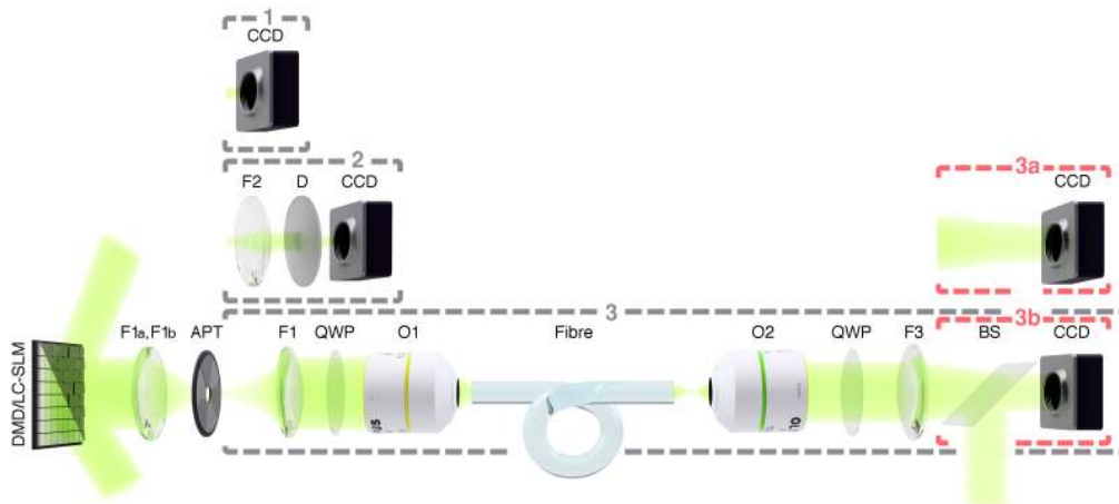
Fig. 1. Modular experimental setup. 1. Ballistic regime. 2. Diffusive regime. 3. MMF with internal(a) or external(b) phase reference. Laser: single-frequency DPSS laser at 532nm (Crystalaser CL532-075-S); LC-SLM (Meadowlark HSPDM512); DMD (VIALUX V-7001); CCD (Basler pia640-210gm); lenses: F1a (Thorlabs AC254-500-A-ML), F1b (Thorlabs AC254-200-A-ML), F2 (Thorlabs AC254-25-A-ML), F3 (Thorlabs AC254-200-A-ML); APT: iris diaphragm (Thorlabs SM1D12D); QWP: quarter-wave plate (Thorlabs WPQ05M-532); D: ground glass diffuser (Thorlabs DG10-1500-MD); Fibre: 30 cm long 0.22 NA multimode fibre (Thorlabs FG050UGA); O1, O2: microscope objectives (Olympus RMS10X, RMS20X); BS: 50:50 non-polarising beamsplitter (Thorlabs BS004).
