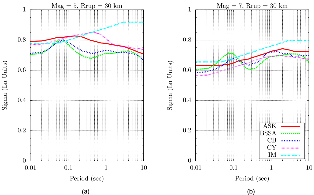
Figure 10. Comparison of the standard deviation for (a) M 5 and (b) M 7 strike-slip earthquakes at a distance of R_{RUP} = 30 km for V_{S30} = 760 m/s.
