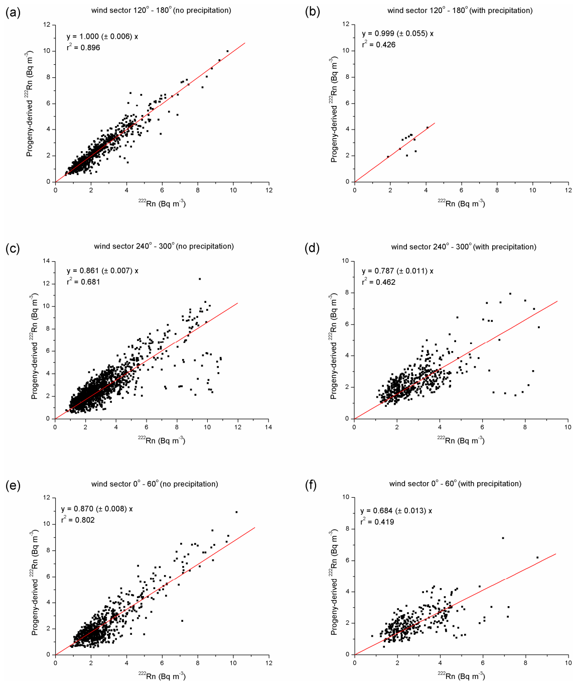
Fig. 7. Correlation between activity concentration of progeny-derived ^{222}\text{Rn} and ^{222}\text{Rn} for the reference sector ( a, b ) and the two sectors influenced by forest cover ( c, d, e, f ), for without precipitation ( a, c, e ) and with precipitation ( b, d, f ) (values in brackets are standard errors of regression parameters). Instrumental background and calibration have been harmonised between detectors.
