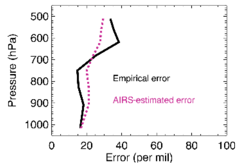
Figure 5. Plot of AIRS error analysis for coincident AIRS and ORACLES \delta D on 31 August 2016, which shows that the empirical error is comparable to the AIRS-estimated error. The empirical error is obtained from the statistics of the satellite–aircraft comparison, while the estimated error is obtained from optimal estimation retrieval theory. Plotted here are the AIRS \delta D-estimated error, also known as AIRS observation error (dashed red line), and the AIRS \delta D empirical error (black line).
