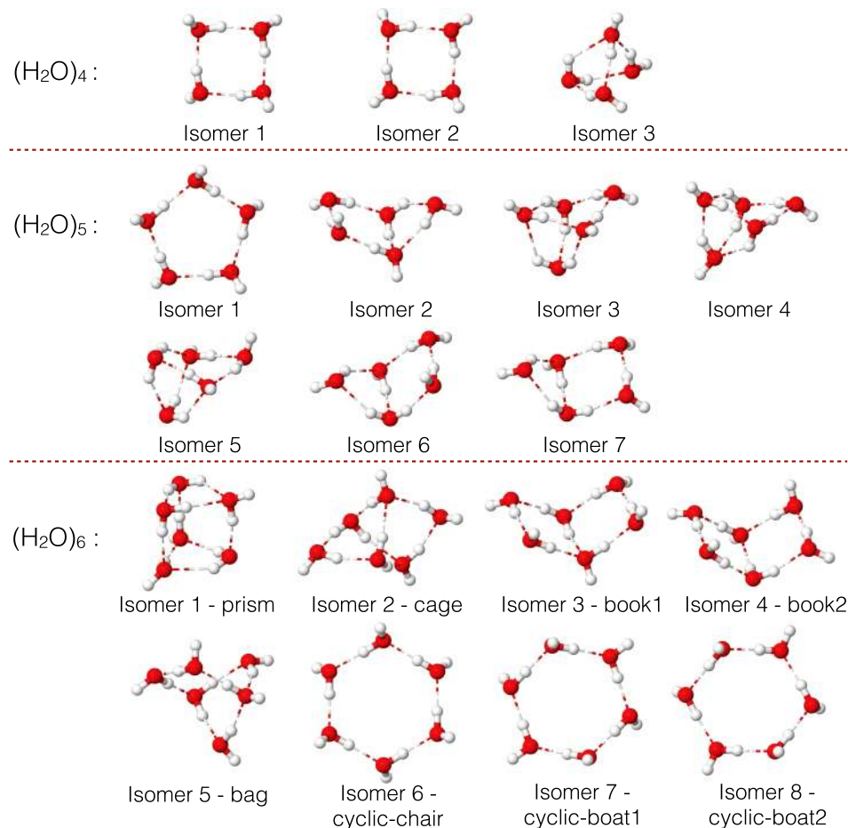
FIG. 4. Isomers of water clusters (H_2O)_n , n = 4, 5, 6 , used for the analysis of the performance of PIP, BPNN, and GAP representations of 2B and 3B energies. Reproduced with permission from Reddy et al. , J. Chem. Phys. 145 , 194504 (2016). Copyright 2016 AIP Publishing LLC.
