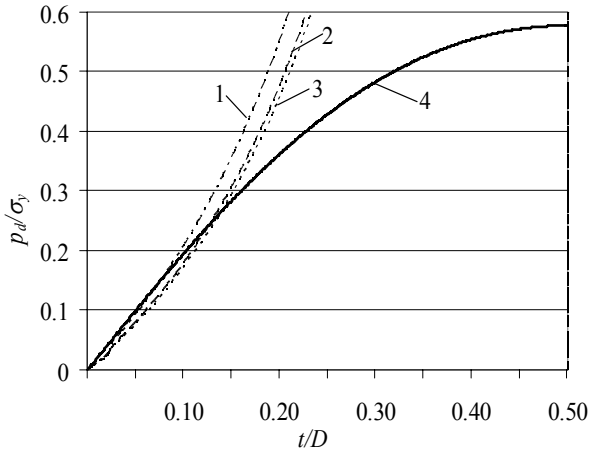
Fig. 5 СНП standard design pressure and Von-Mises yield pressure results: 1 - СНП “Low safety class”; 2 - СНП “Normal safety class”; 3 - СНП “High safety class”; 4 - Von-Mises criteria for thick pipes with open valves
