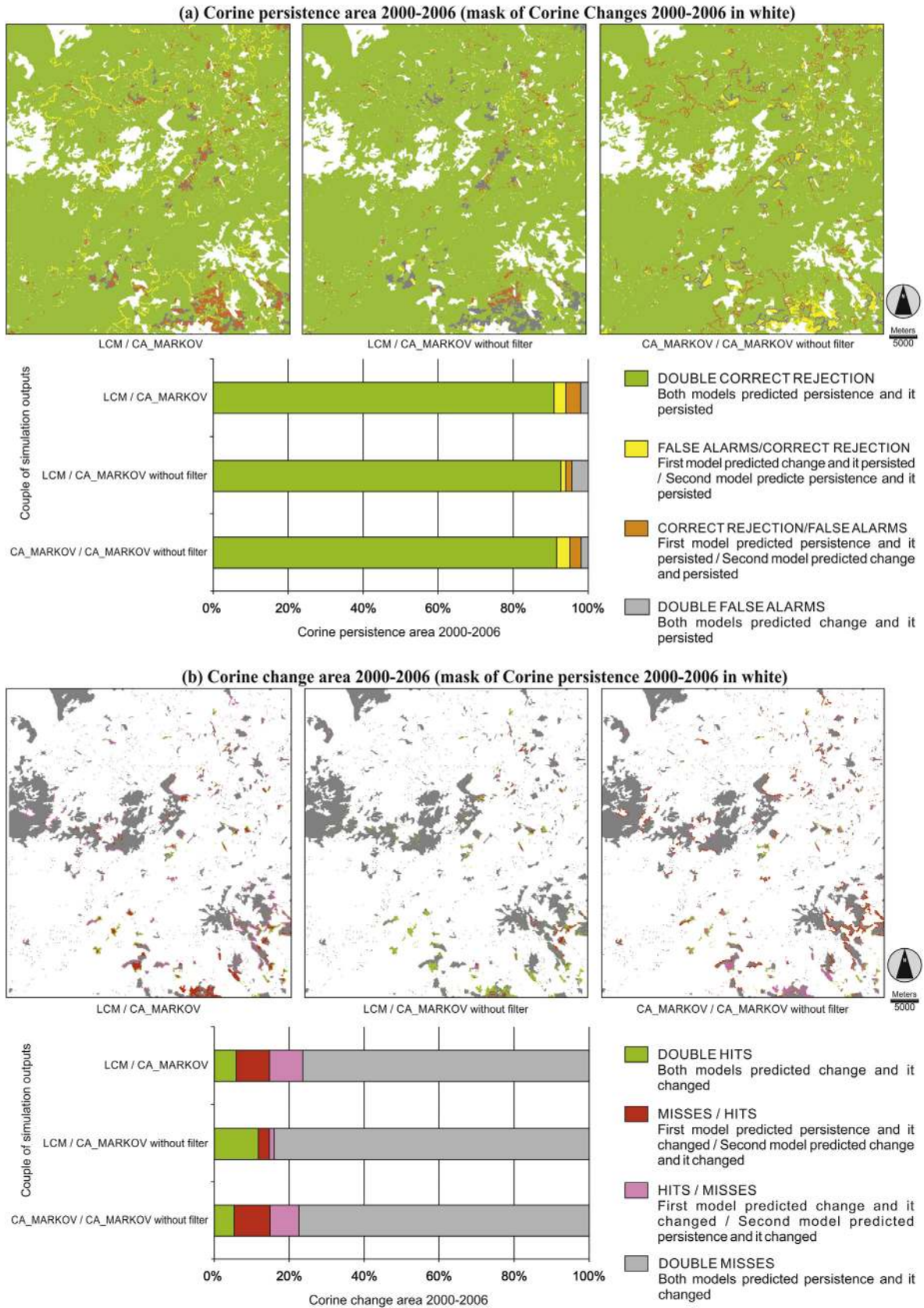
Fig. 5. Pattern validation during 2000–2006 by overlaying pairs of simulation outputs: LCM versus CA_MARKOV, LCM versus CA_MARKOV without filter, and CA_MARKOV versus CA_MARKOV without filter. (a) Corine persistence area. (b) Corine change area.
