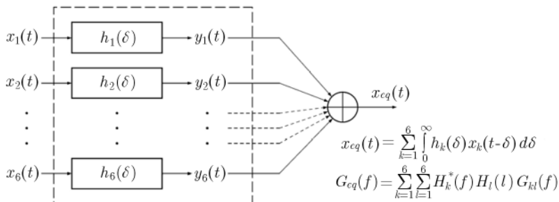
Fig. 2. Interpretation of the damage parameter x_{eq}(t) as an output signal from the physical system with pulse transition functions h_k(\delta) , k = 1, \dots, 6 where signals x_k(t) , k = 1, \dots, 6 were introduced to its input
