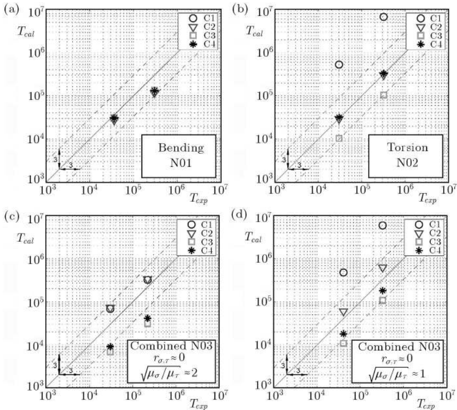
Fig. 7. Comparison of the calculated T_{cal} and experimental T_{exp} time to failure for loading cases N01-N04
