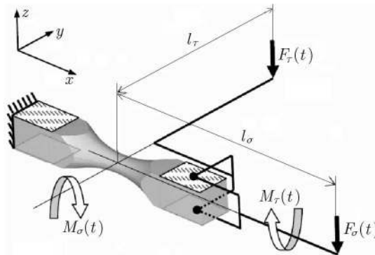
Fig. 6. Geometry of the specimen with scheme of the loading presented by Niesłony and Macha (2007)
