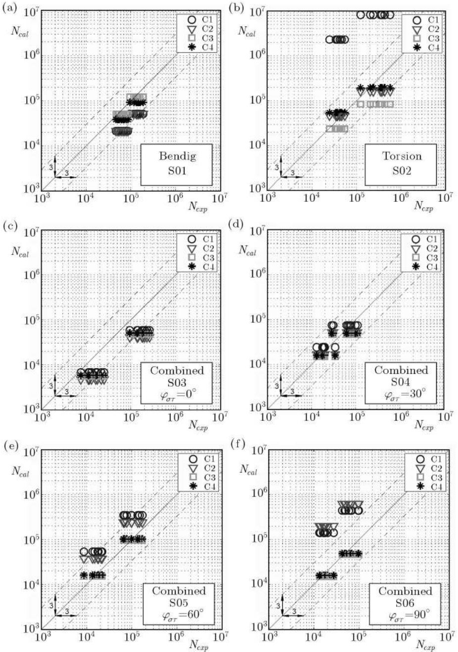
Fig. 5. Comparison of the calculated N_{cal} and experimental N_{exp} cycles to failure
