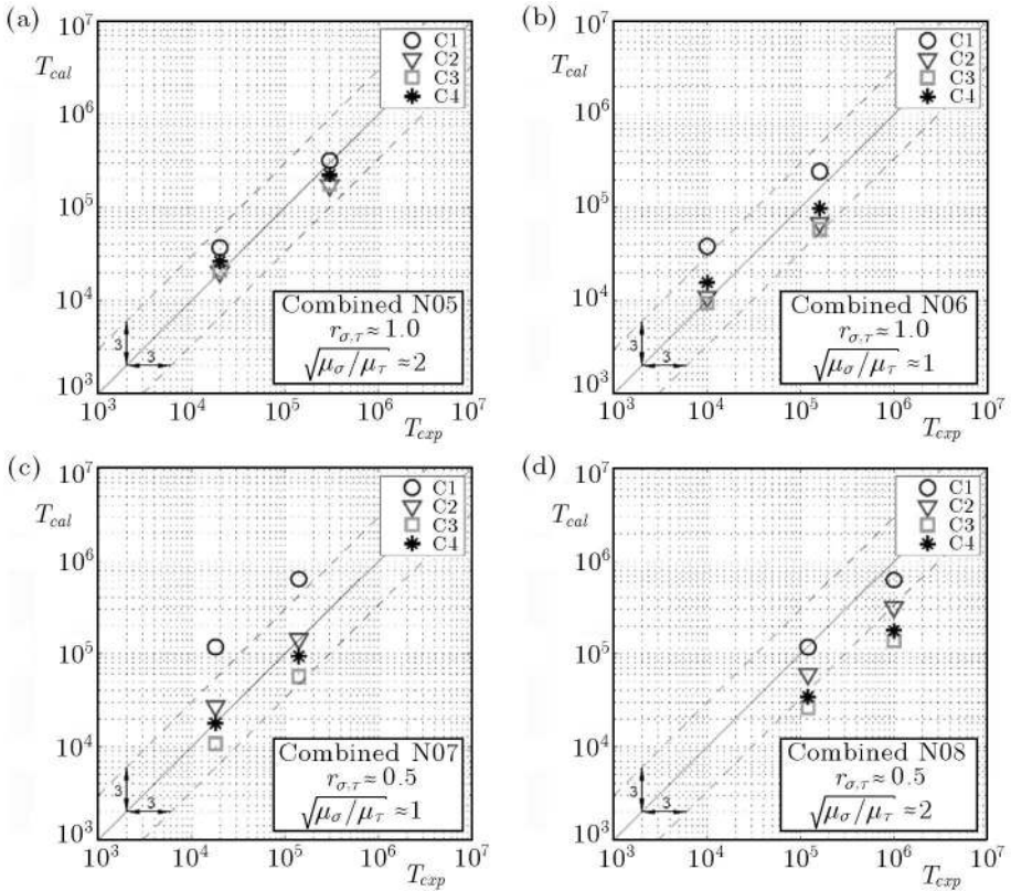
Fig. 8. Comparison of the fatigue life calculated according to the four criteria C1-C4 with the experimental life, loading cases N05-N08
