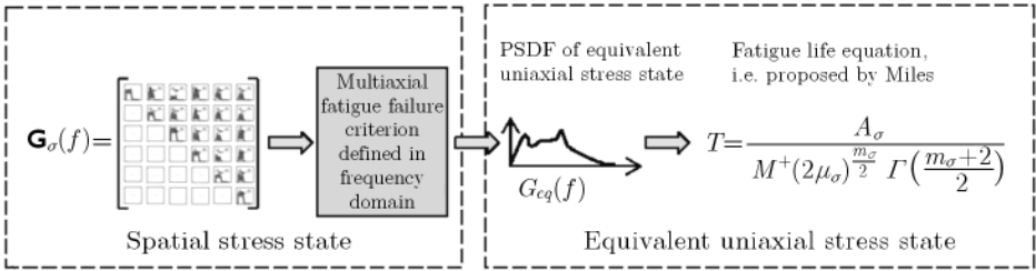
Fig. 1. Flow chart for calculation of fatigue life using spectral method under multiaxial random loading
