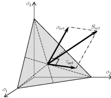
Fig. 3. Normal and shear stresses acting on the octahedral plane
