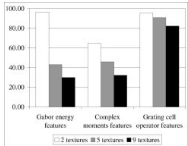
Fig. 4. Percentages of correctly classified pixels using the fuzzy c-means classification algorithm.
