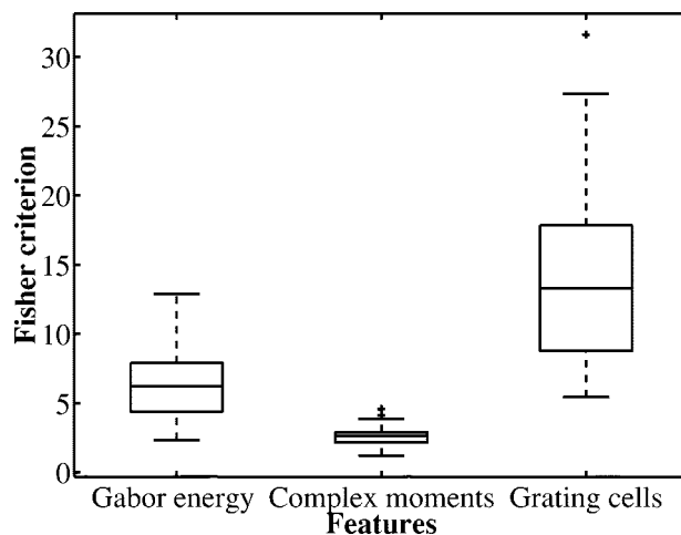
Fig. 2. Boxplot representation of the distribution of the Fisher criterion values obtained with different texture operators.
