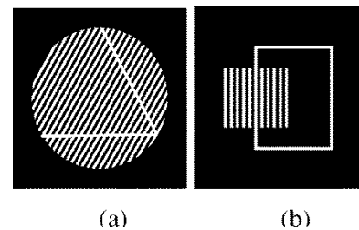
Fig. 7. Examples of suppression of contour perception by a grating: (a) the side of the triangle that is parallel to the bars of the grating does not pop out as the other two sides do and (b) part of the contour of the rectangle is “lost” in the grating [56].
