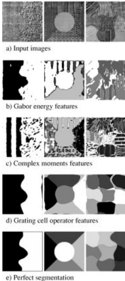
Fig. 3. Segmentation results obtained with the fuzzy c-means classification algorithm for texture images containing two, five, and nine oriented textures.
