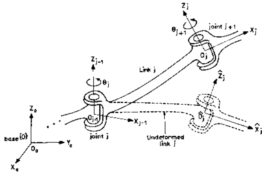
Figure 1: Coordinate systems for the flexible link j
