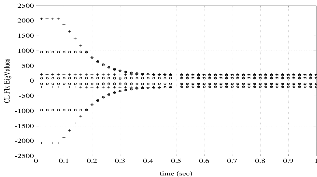
Figure 9: Time history of mode 1 closed-loop imaginary eigenvalues of flexible variables corresponding to links 2 and 3. ( o : assumed modes model, + : finite element model )
