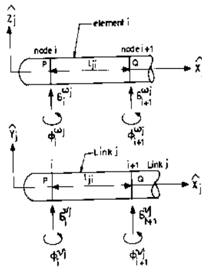
Figure 2: A beam element with nodal displacements in link j
