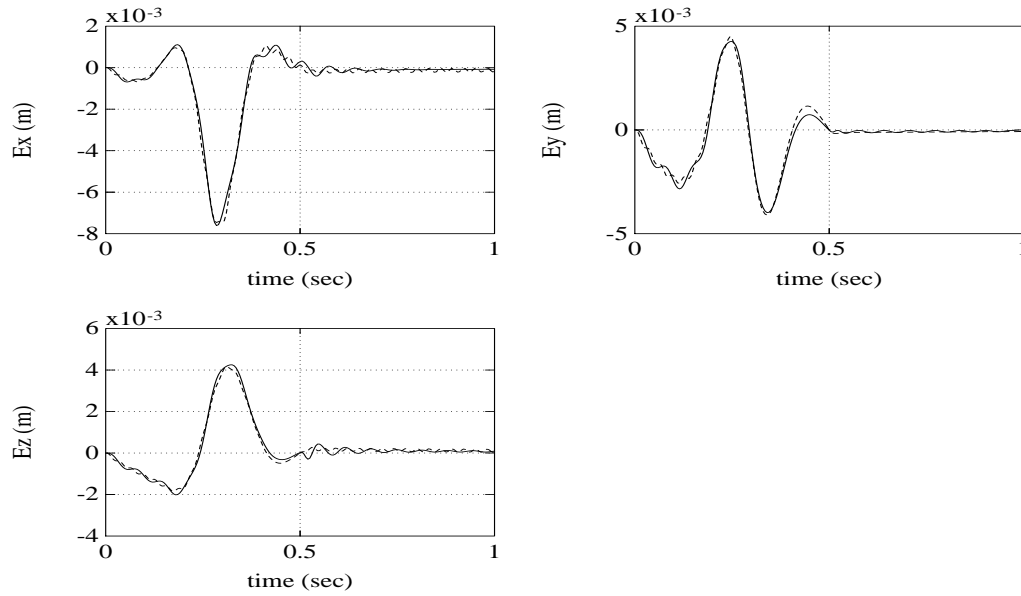
Figure 6: Time history of the end-effector position errors. (— : assumed modes model, - - - : finite element model)
