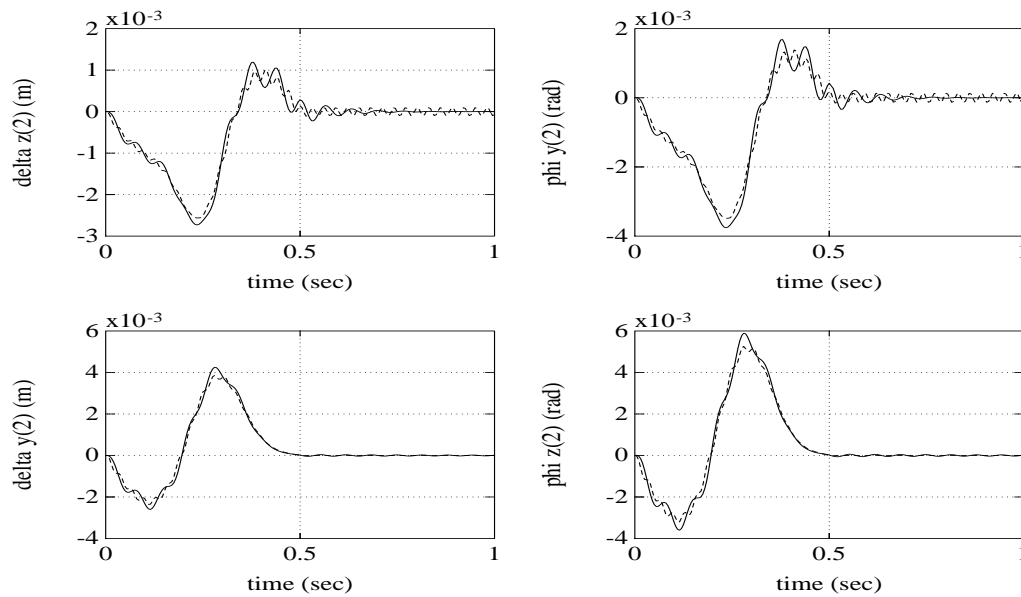
Figure 7: Time history of flexible deflection and rotation of the in-plane and out-of-plane components, at the tip of link 2. (— : assumed modes model, - - - : finite element model)
