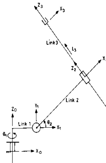
Figure 3: Flexible spherical (RRP) manipulator
