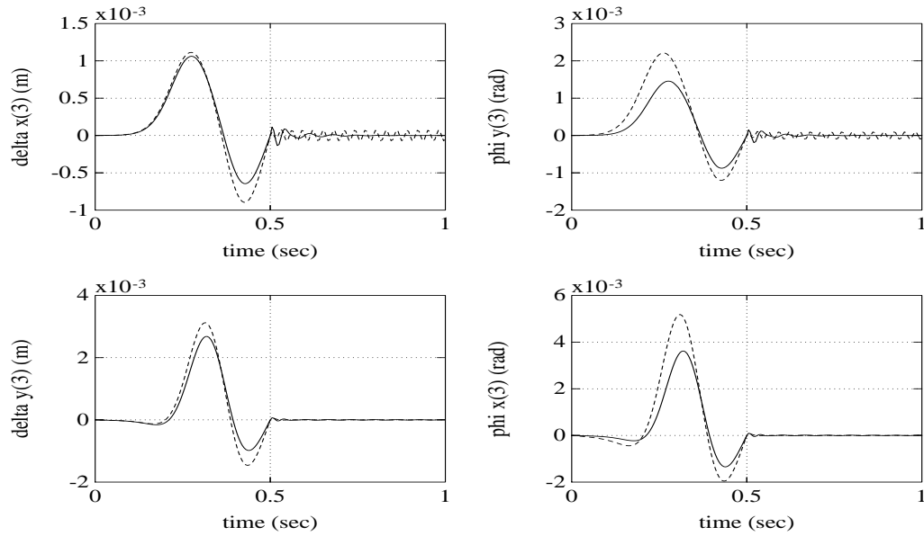
Figure 8: Time history of flexible deflection and rotation of the in-plane and out-of-plane components, at the tip of link 3. (— : assumed modes model, - - - : finite element model)
