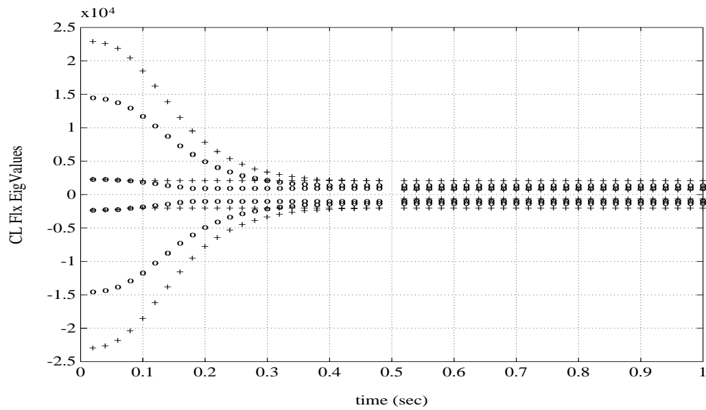
Figure 10: Time history of mode 2 closed-loop imaginary eigenvalues of flexible variables corresponding to links 2 and 3. ( o : assumed modes model, + : finite element model )
