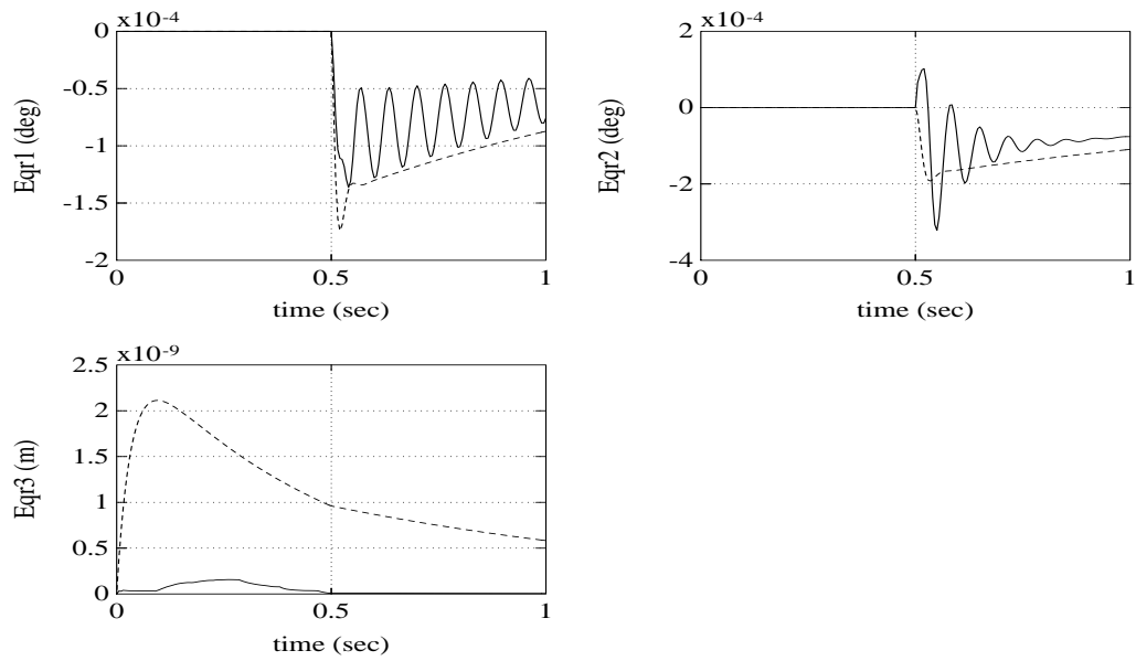
Figure 5: Time history of the joint position errors. (— : assumed modes model, - - - : finite element model)
