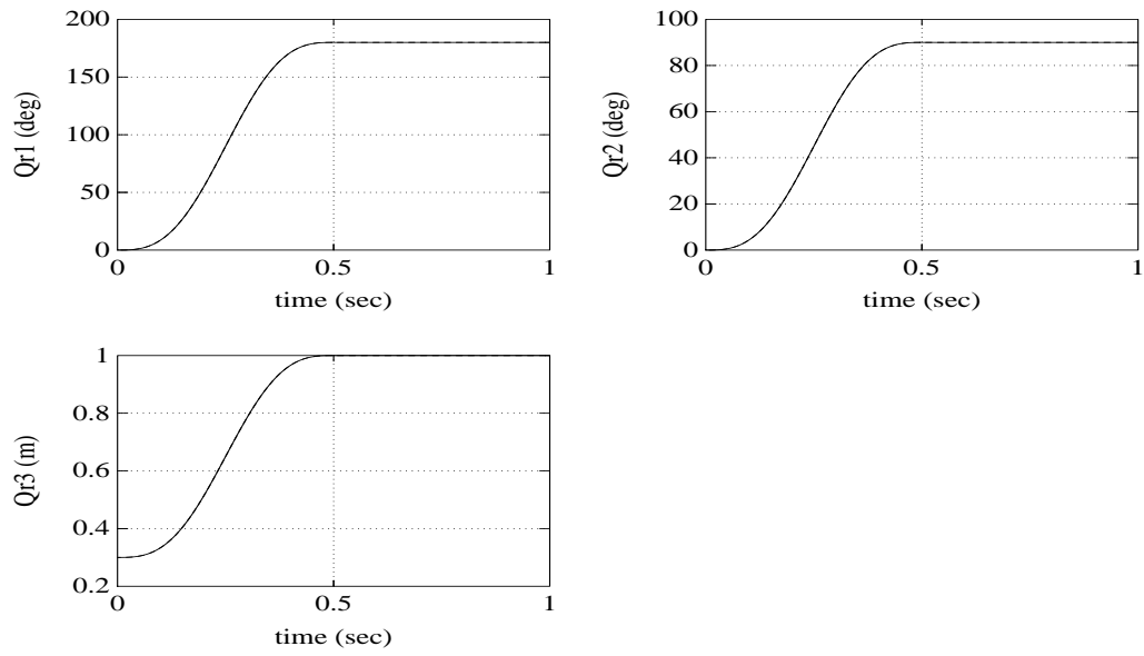
Figure 4: Desired and actual joint position trajectory
