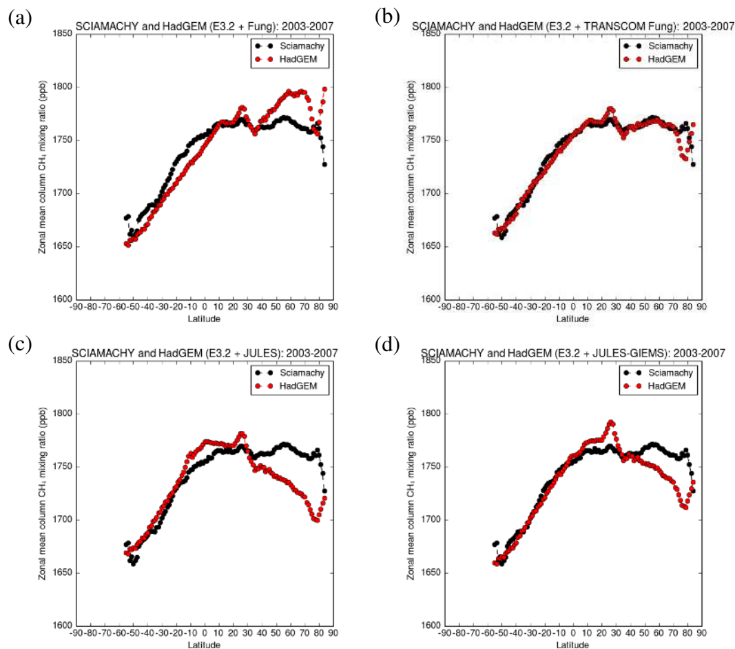
Figure 9. Comparisons of the latitudinal distribution of the average atmospheric column methane mixing ratio between the years 2003 and 2007, as derived from monthly regrided SCIAMACHY data and from the HadGEM2 runs using the FUNG (a), TRANSCOM-FUNG (b), JULES (c) and JULES-GIEMS (d) wetland emission inventories and the EDGAR v3.2 (E3.2) anthropogenic methane emission time series, sampled at co-located space and time points. Note that the SCIAMACHY data between 60 and 90° S have been removed because of their sparsity and quality.
