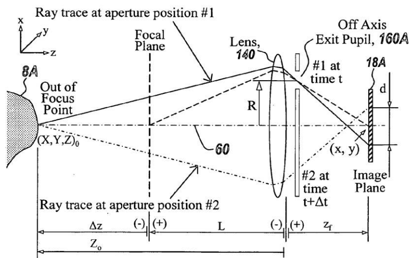
Figure 4. Diagram of Aperture Mechanism 54
