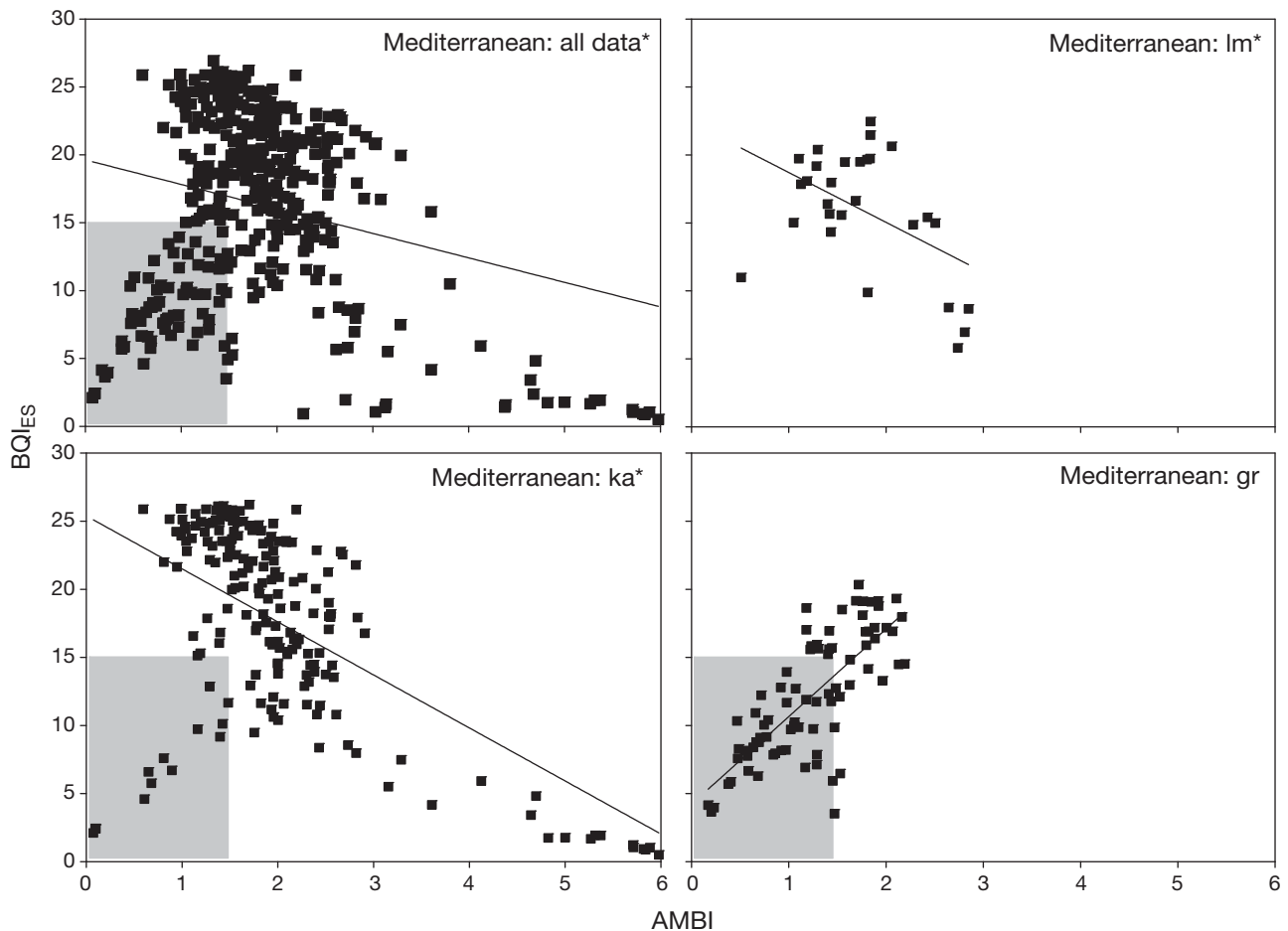
Fig. 8. Relationships between AMBI and BQI ES in the Mediterranean. Data are provided for the whole Mediterranean and 3 individual data sets (see Table 1). *Significant ( p < 0.05 ) negative correlation (for the subarea or the individual data sets) between AMBI and BQI ES . Shaded rectangles in the bottom left of the Mediterranean, ka and gr graphs delimit stations with a low AMBI (<1.5) and BQI ES (<15) (see 'Results-Comparisons between AMBI and BQI ES ' for details)
