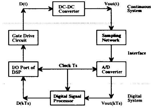
Fig. 4. Block diagram of DSP controlled forward converter
