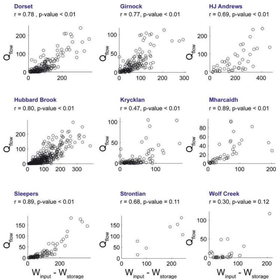
Figure 5. Total quickflow ( Q_{flow} , mm) versus effective water input ( W_{input} - W_{storage} , mm) in the nine North-Watch catchments for snowmelt-driven events. The Spearman rank correlation coefficient ( r_{Spearman} , abbreviated as 'r') and its associated p-value are reported
