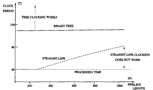
Fig. 11. Straight-line vs tree clocking schemes: N = 100 to 1000.
