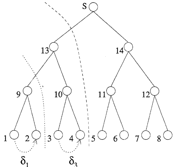
Fig. 5. Clock skew in a binary tree.
