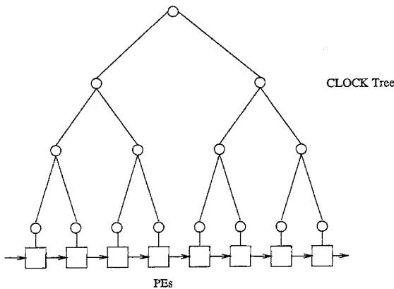
Fig. 1. Tree clocking scheme.
