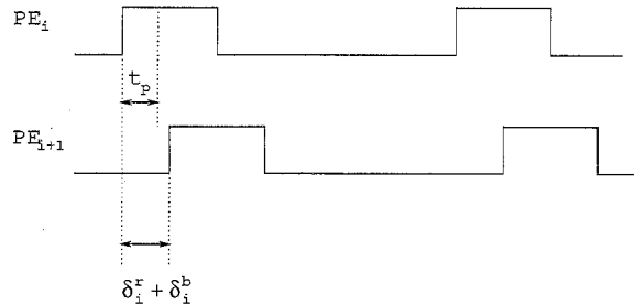
Fig. 4. Type-2 Failure: the input to PE i+1 changes before it latches its proper input.
