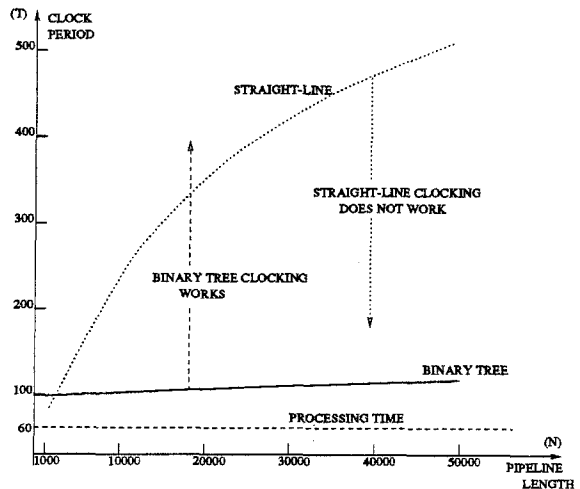
Fig. 12. Straight-line vs tree clocking schemes: N = 1000 to 50000.
