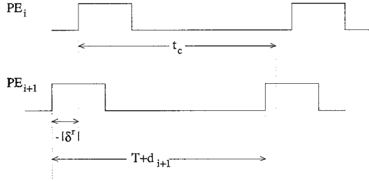
Fig. 3. Type-1 Failure: the output of PE i appears too late to be latched by PE i+1 .
