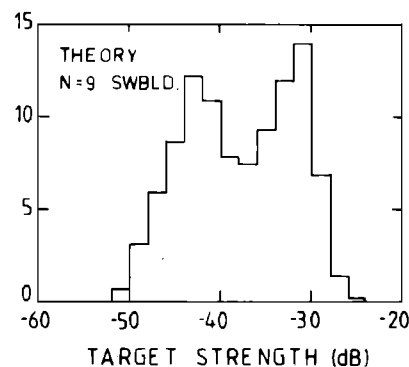
FIG. 4. Length-frequency distribution for trawl haul 1 and TS pdf's from dual-beam and split-beam measurements in sample 1 and from theoretical calculation based on nine swimbladders, the catch data for the trawl, and the tilt angle distribution N(2,5) .
