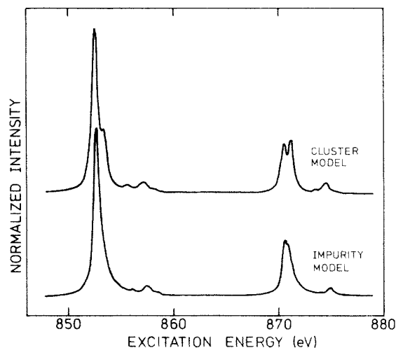
FIG. 7. Cluster model and impurity model compared for the case of NiI_2 ( \Delta = 1 eV).
