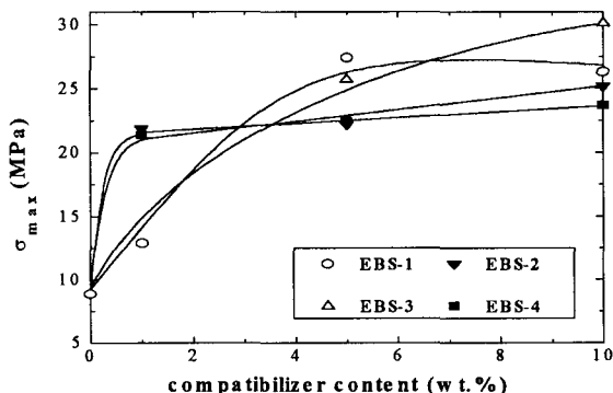
Figure 2. Blend tensile strength versus compatibilizer content for different segmented EB(PS\text{-}block\text{-}EB)_n block copolymers.
