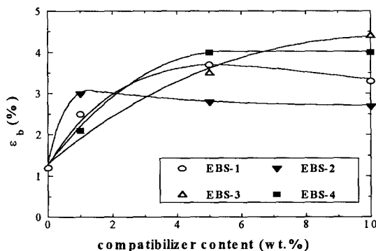
Figure 1. Elongation at break of a (10/90) LDPE/PS blend versus compatibilizer content for various segmented block copolymers.
