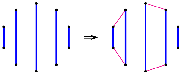
Figure 3: A 5-edge perfect matching with no disjoint compatible perfect matching.
