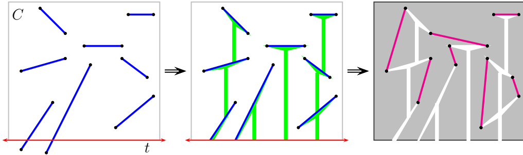
Figure 2: Second proof of Lemma 5.
