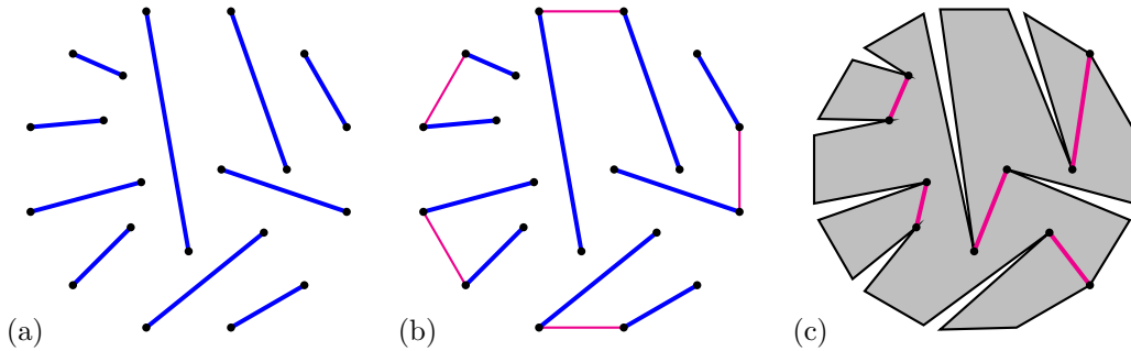
Figure 6: Proof of Theorem 13: (a) a convex-hull-connected set M of segments, (b) the set B of alternate gaps, (c) the polygon P and matching Q .
