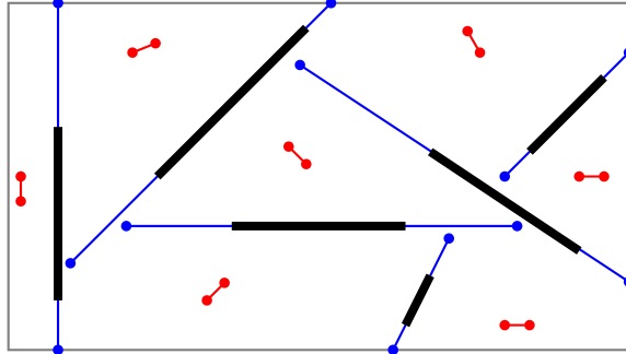
Figure 4: The blue and red segments form an odd perfect matching with no disjoint compatible perfect matching.
