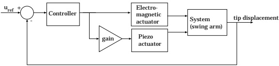
Figure 4: actuation scheme of the swing arm
