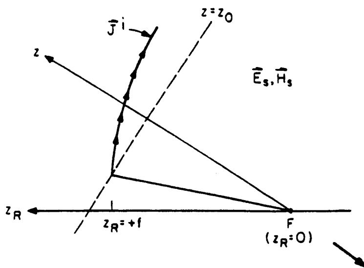
(a) Induced current \vec{J}^i on the reflector surface produces scattered fields \vec{E}_s, \vec{H}_s .
