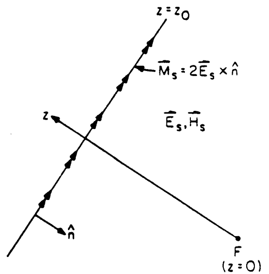
(b) Equivalent magnetic current \vec{M}_s produces scattered fields \vec{E}_s, \vec{H}_s for z less than z_0 .
