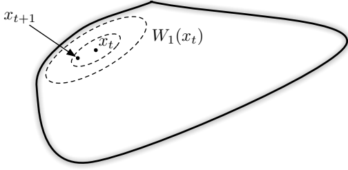
Figure 1: The Dikin ellipsoid W_1(\mathbf{x}_t) at \mathbf{x}_t . The next minimum is guaranteed to lie in its scaled version W_{4n\eta}(\mathbf{x}_t) .
