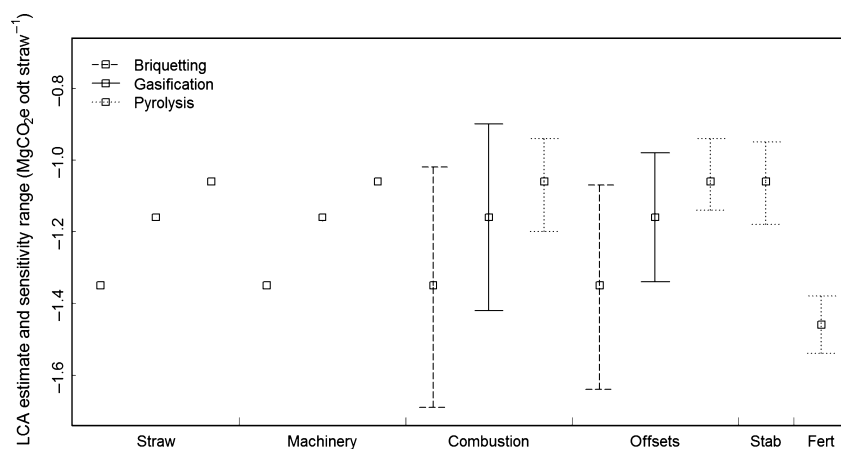
Fig. 5 Baseline carbon abatement estimates (MgCO 2 e abated odt per straw) and sensitivity analyse for key parameters determining the carbon abatement potential of briquetting, gasification and pyrolysis. Ranges are produced by independently varying key parameters ( x -axis) by \pm 20\% and recording the impact on overall carbon abatement potential.
